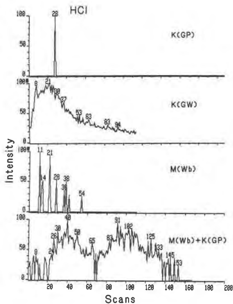
Fig. 3. SIR traces of HCl + .
