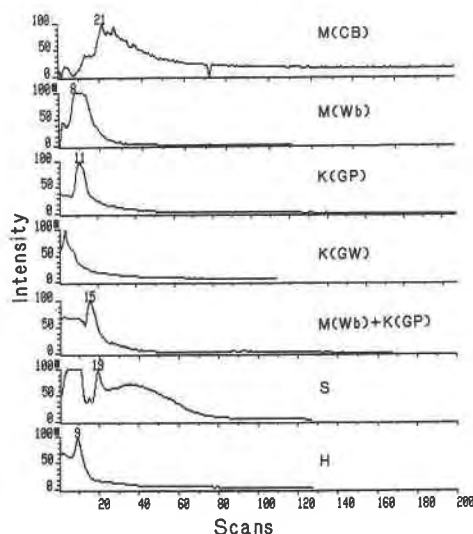
Fig. 5. SIR traces of OH + ( m/z = 17.0027).
