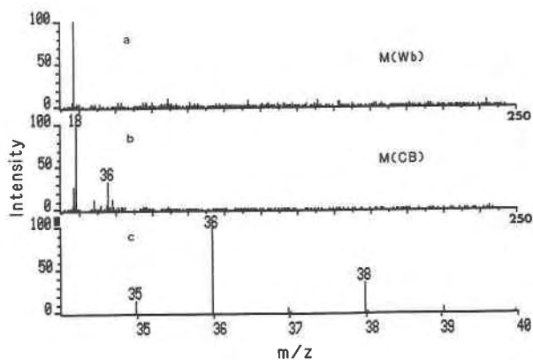
Fig. 1. Mass spectra of volatiles from (a) M(Wb), m/z = 10 –250; (b) M(CB), m/z = 10 –250; (c) M(CB), m/z = 34 –40.
