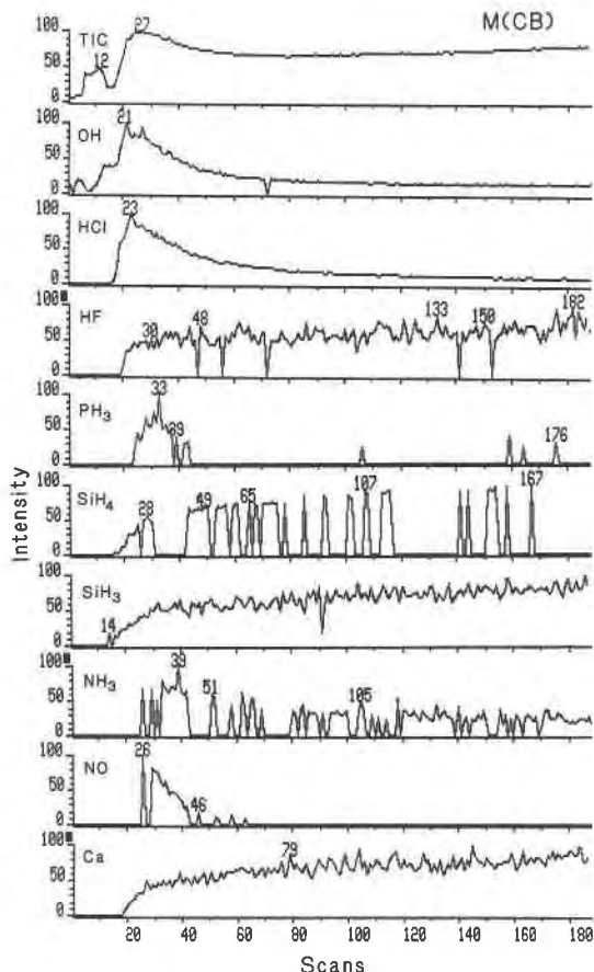
Fig. 2. SIR traces of selected volatiles derived from M(CB).
