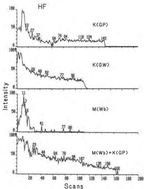
Fig. 4. SIR traces of HF + .
