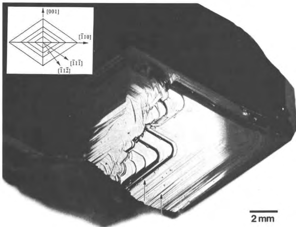
Fig. 2. Growth steps (arrows) on a \{110\} surface of Eden Mills grossular ( \text{Gr}_{90}\text{And}_6\text{Alm}_4 ) seen in reflected light.
