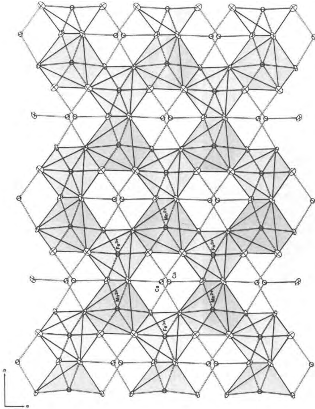
Fig. 4. Projection of the dioctahedral interlayer of franklinfurnaceite on a plane rotated by 5^\circ from (001), showing the rings of alternating \text{Mn}^{2+}(\text{OH})_6 and \text{Fe}^{3+}(\text{OH})_6 octahedra and the Ca atoms situated above and below vacant octahedral sites. Only three of the six Ca-O bonds are shown. The \text{Mn}^{2+} sites contain minor Mg and Zn and the \text{Fe}^{3+} sites contain minor Al.
