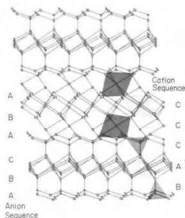
Fig. 2. Projection of the franklinfurnaceite structure on a plane 5° from (010), showing the anion- and cation-stacking sequences.
