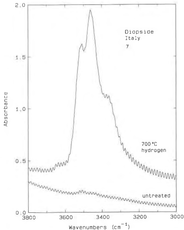
Fig. 6. Ferrian diopside (Italy) in \gamma polarization, before (bottom) and after (top) heating in H_2 at 700 °C for 6 h, normalized to 1-mm thickness. The absorption intensities increase weakly in the other optical directions. Sample thickness 0.20 mm, (010) section. The high-frequency sinusoidal modulation is due to interference fringes, not sample absorption.
