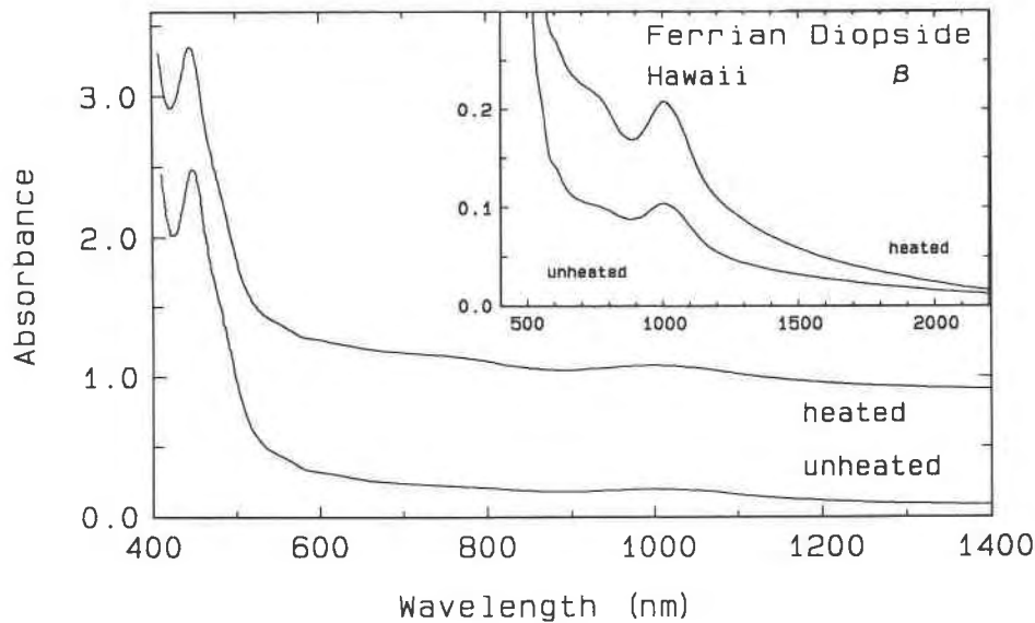
Fig. 9. Spectra of ferrian diopside (no. 21, Hawaii) in \beta polarization before and after heating in hydrogen at 700 °C for 6 h. The \text{Fe}_{M(2)}^{3+} band at 1020 nm increases during treatment. The band at 450 nm has been assigned to tetrahedral \text{Fe}^{3+} (Bell and Mao, 1972). The y scale has been expanded in the inset figure. Plotted thickness: 100 \mu\text{m} .
