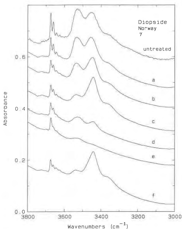
Fig. 4. Polarized \gamma spectra from 1-atm heating experiments conducted on the Norwegian diopside. All spectra normalized to 1-mm thickness. (a) H 2 , 600 °C, 6 h; (b) H 2 , 750 °C, 6 h; (c) H 2 , 825 °C, 6 h; (d) air, 600 °C, 6 h; (e) air, 700 °C, 14 h; (f) H 2 , 600 °C, 6 h. The spectra represent successive experiments performed on the same sample. Crystal thickness 0.61 mm.
