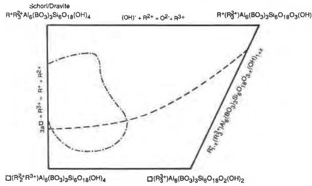
Fig. 1. Diagram showing the substitutional relationships between schorl or dravite and the hypothetical proton and alkali-deficient series, R_{1-x}R_3^+Al_6(BO_3)_3Si_6O_{18}O_{3-x}(OH)_{1+x} , which is defined by proton-deficient [R^+R_3^+Al_6(BO_3)_3Si_6O_{18}O_3(OH)] and alkali cation-free [R^2+R_3^+(BO_3)_3Si_6O_{18}O_2(OH)_2] end-members. The dashed line shows the extent of substitution in natural samples reported by Foit and Rosenberg (1977), and the dot-dashed line gives the extent of substitution in the Jack Creek and Ben Lomond schorls.
