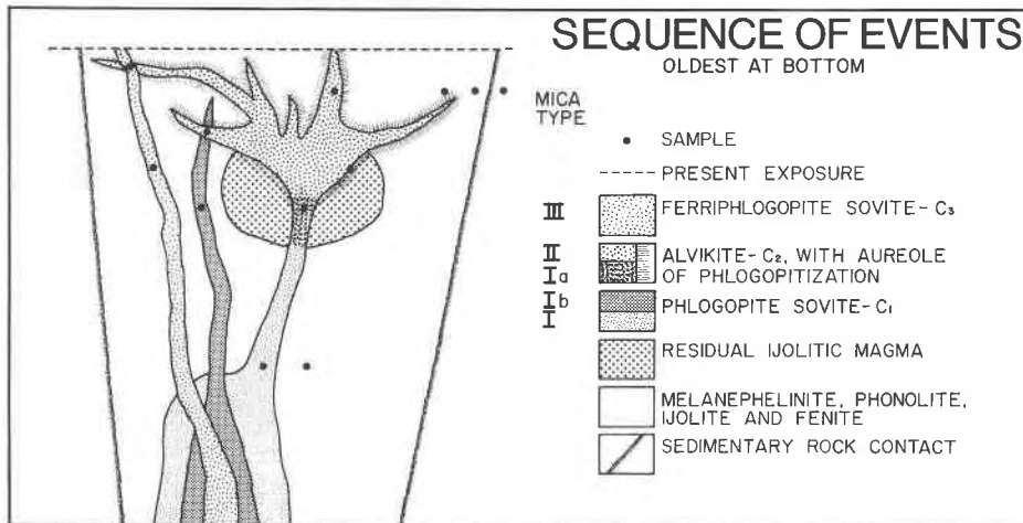
Fig. 7. Schematic representation of magmatic activity in the Potash Sulphur Springs complex between the time of phlogopite sovite (C 1 ) formation and later solidification of ferriphlogopite sovite (C 3 ). This period is interpreted to have preceded the formation of syenite. Relative ages of magmatic units are indicated by crosscutting. Dots noted as sample points represent sample coverage of the geologic units and crosscutting relationships discussed in text. Mica types are noted adjacent to the units in which they are found.
