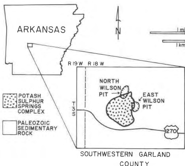
Fig. 1. Location of the Potash Sulphur Springs complex. Current exposure of the alkalic complex is within a folded and faulted sedimentary country-rock section that is dominated by massively bedded chert.
