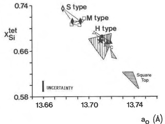
Fig. 3. Mole fraction of Si in the tetrahedral site ( X_{Si} ) of analcime versus cubic cell constant a_0 . Solid symbols represent the six samples from this study: dot = P-type analcime SAY-104; star = L-type analcime R-36; diamonds = S-type samples ST and WMT; triangles = H-type analcimes BPF and KH. Open symbols and letters are data from the literature: open diamond = S-type analcime; open squares = M-type analcimes; and open triangles = H-type analcimes (Coombs and Whetten, 1967). Suggested P-type analcimes from the literature: C = Crowsnest Formation (Wilkinson, 1968); X = Queensland analcimite (Wilkinson, 1977); vertically ruled field outlines analcimes from the Azerbaijan, Iran, tephrites, phonolites, and analcimite (Comin-Chiaramonti et al., 1979); stippled field = analcimite and analcime phonolites from the Highwoods Mountains and analcime tinguaites from the Otago Harbor (Wilkinson, 1968); horizontally ruled field = three analcimes from the Square Top Intrusion (Wilkinson, 1965). Error bar indicates uncertainties from Table 2.
