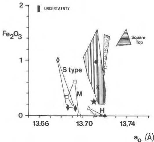
Fig. 4. \text{Fe}_2\text{O}_3 content of analcime (wt%) versus cubic cell constant a_o . Symbols as in Fig. 3.
