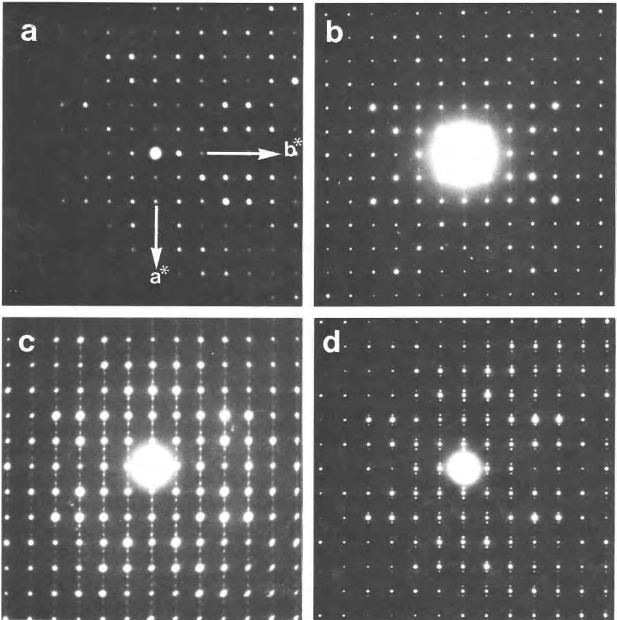
Fig. 2. Electron-diffraction patterns of krupkaite-aikinite minerals down [001]: (a) krupkaite, Balls mine, Utah (specimen no. 9); no superlattice intensity visible along a^* . (b) Aikinite, Lime Creek mine, Canada (specimen no. 1); note streaking along a^* owing to stacking disorder. (c) Aikinite, Dobsina, Czechoslovakia (specimen no. 4); streaked 3 \times superlattice reflections along a^* due to the intergrowth of friedrichite and krupkaite units in aikinite. (d) Lindströmite, Silver Miller mine, Canada (specimen no. 6). The sharp, well-formed 5 \times superlattice reflections characteristic of the minerals are clearly visible along a^* .
