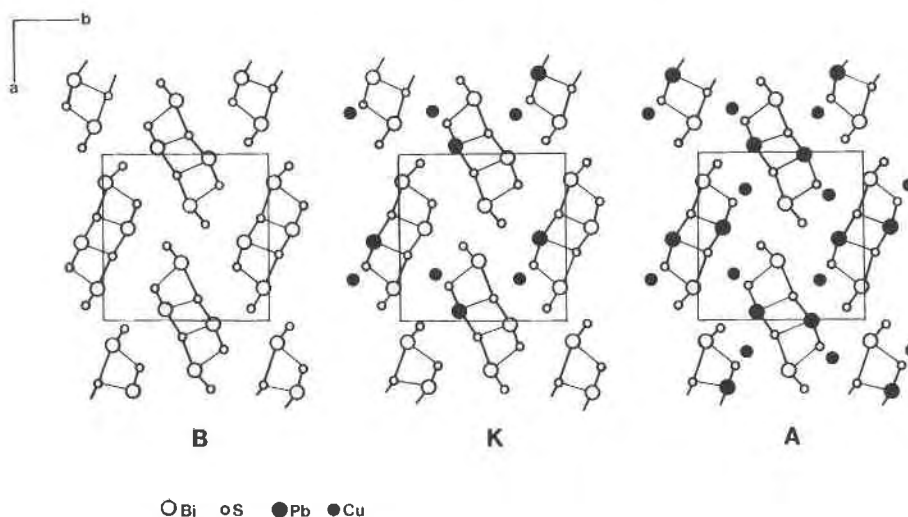
Fig. 1. The structures of bismuthinite (B), krupkaite (K), and aikinite (A). The bismuthinite structure (B) can be considered as the archetype of the group, the structure of the other minerals in the series being derived by ordered cation substitution and insertion. The structure is composed of quadruple \text{Bi}_4\text{S}_6 chains, in which half the Bi is in threefold coordination and the other half is in fivefold coordination, forming \text{Bi}_4\text{S}_6 ribbons, there being two such ribbons per unit cell. Krupkaite (K) is derived from bismuthinite by replacing one-quarter of the \text{Bi}^{3+} by \text{Pb}^{2+} and insertion of \text{Cu}^+ into half of the available tetrahedral sites in an ordered fashion. In aikinite, half the \text{Bi}^{3+} cations are replaced by \text{Pb}^{2+} , and all four tetrahedral sites are occupied by Cu. The structures of the other intermediate members are composed of ordered intergrowths of bismuthinite (B), krupkaite (K), and aikinite (A) ribbons.
