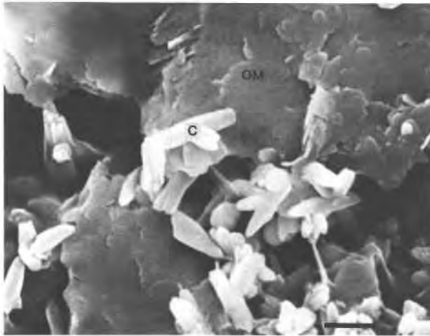
Fig. 1. Scanning electron micrograph of submicroscopic coffinite crystals in remnant primary ore. Note interpenetrating coffinite crystals (C). Matrix is a mixture of clay minerals and amorphous organic matter (OM). Sample 4-1933. Scale bar = 1 \mu\text{m} .
