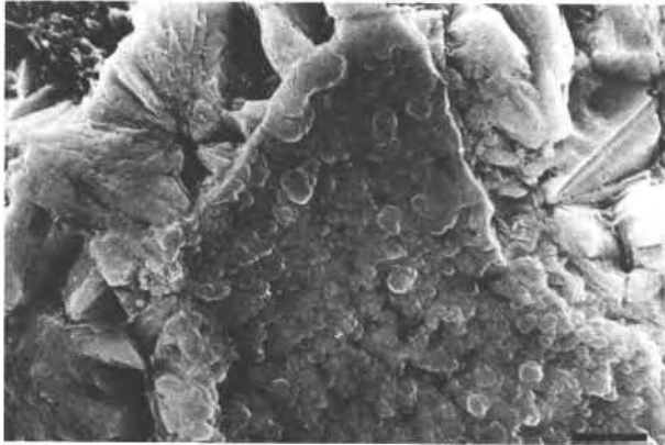
Fig. 6. Scanning electron micrograph of coffinite and associated siliceous microspheres containing major U, Ti, Si, and/or traces of other elements. Sample 7-3260. Scale bar = 5 \mu\text{m} .
