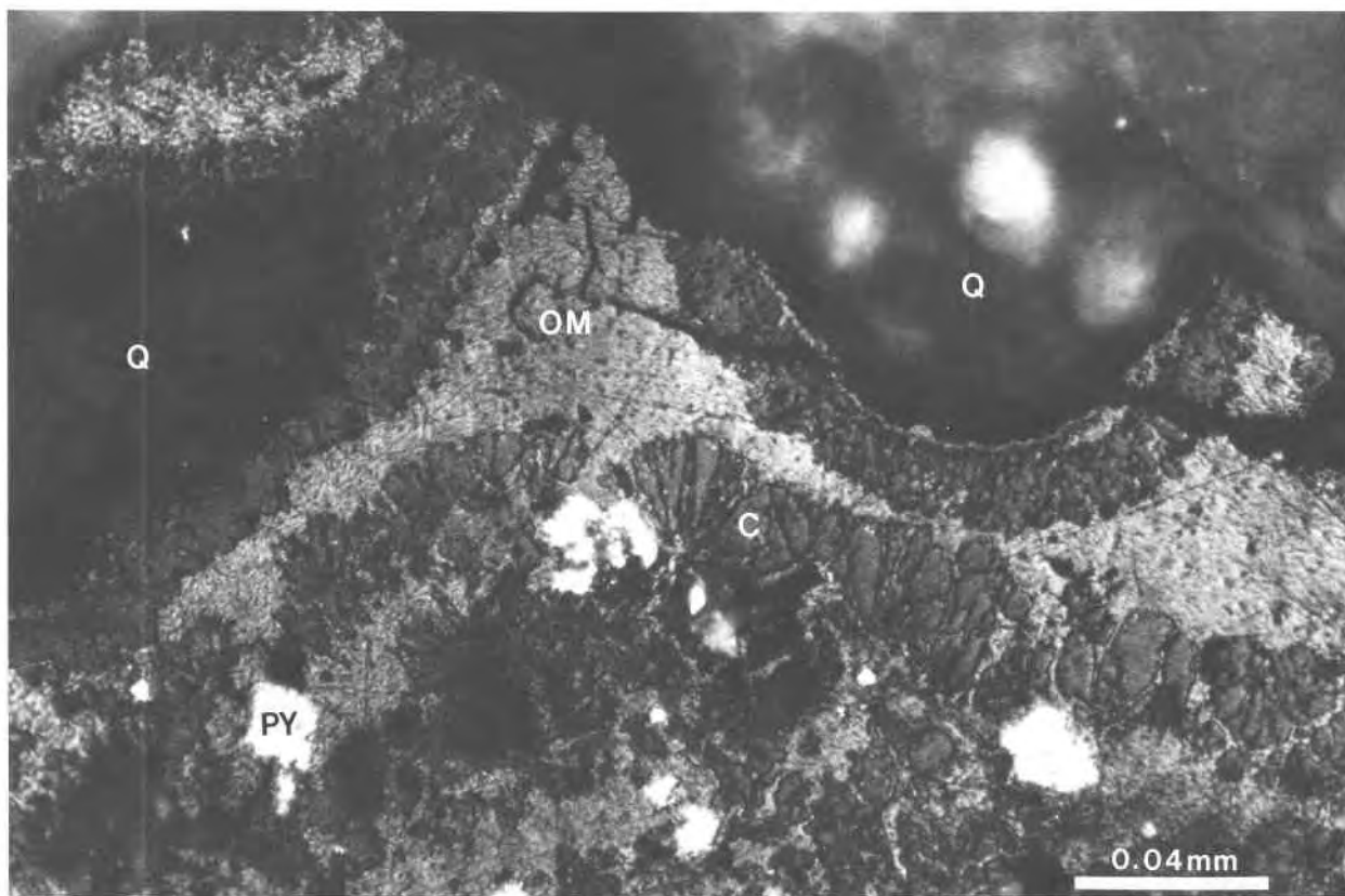
Fig. 3. Photomicrograph of coffinite (C) textures in Nose Rock ore. Q, quartz; PY, pyrite. Organic matter (OM) contains traces of U and other elements. Direct reflected light, oil immersion.
