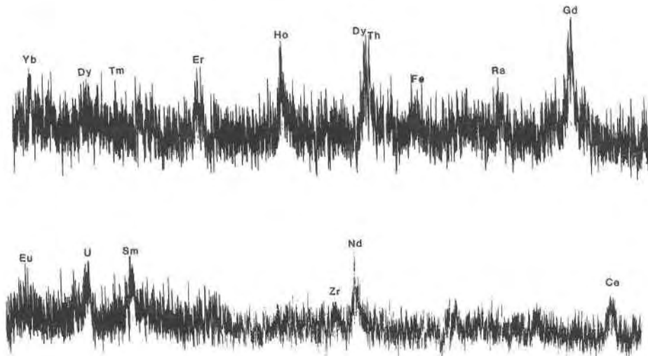
Fig. 5. Expanded wavelength-dispersive spectrum showing the L\alpha peaks of rare-earth elements in coffinite. Spectrum reads from upper left to lower right: Yb (7.41 keV) to Ce (4.84 keV). LiF spectrometer; 15 kV; sample current, 10 nA; time constant, 1.5 s. Sample 7-3185.
