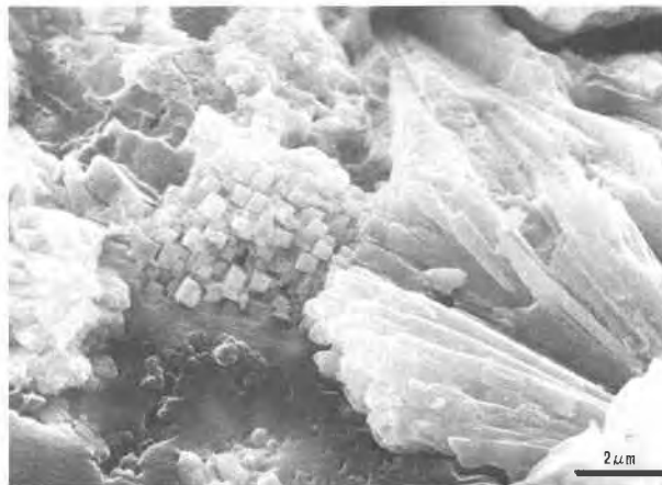
Fig. 4. Scanning electron micrograph of clusters of elongate coffinite crystals with square cross sections. Sample 7-3260.
