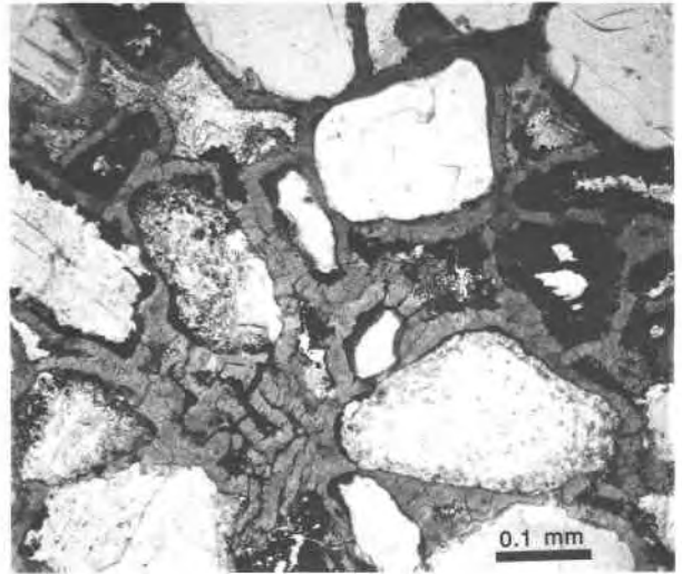
Fig. 2. Photomicrograph of colloform aggregates of coffinite crystals (gray) rimming framework grains. Black material is primary carbonaceous ore and pyrite. Plane-polarized light. Sample H26-22.
