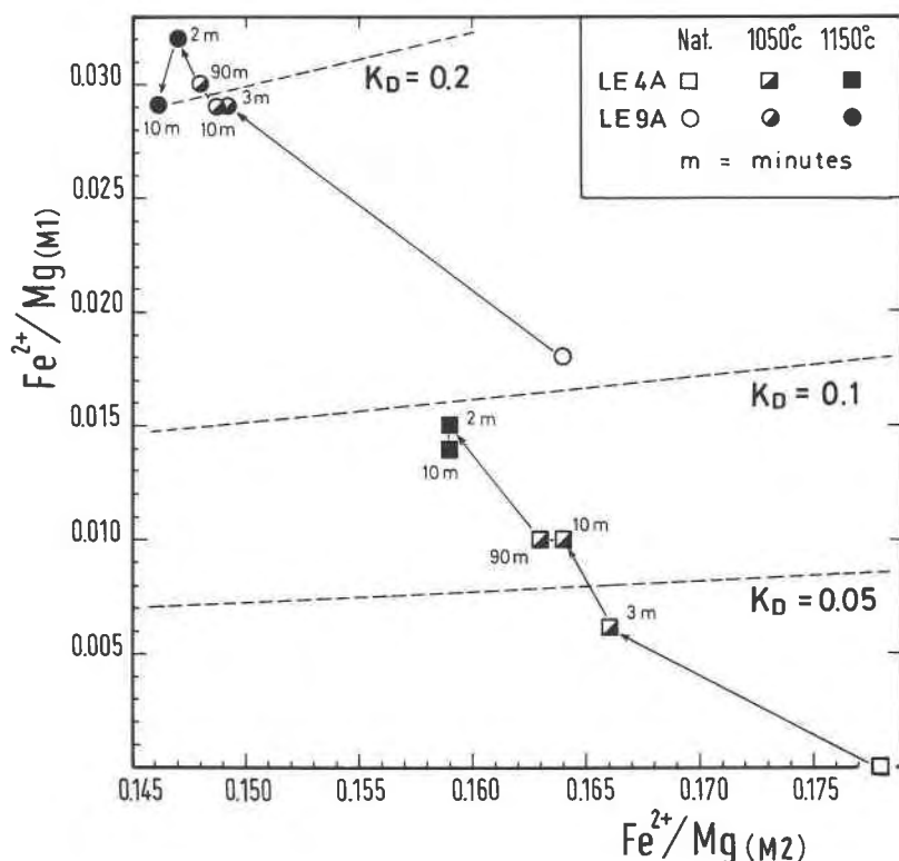
Fig. 1. Relationship between \text{Fe}^{2+}/\text{Mg} on the M2 site and \text{Fe}^{2+}/\text{Mg} on the M1 site for natural and heated Le4A and Le9A crystals. Dashed lines: constant distribution coefficients, K_D ( K_D = \text{Fe}_{M1}^{2+}\text{Mg}_{M2}/\text{Fe}_{M2}^{2+}\text{Mg}_{M1} ).
