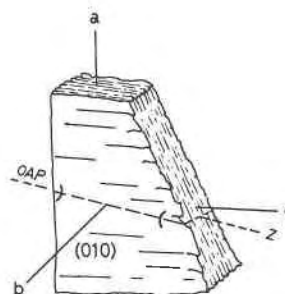
Fig. 2. An idealized sketch of a geigerite crystal showing the optical orientation.
