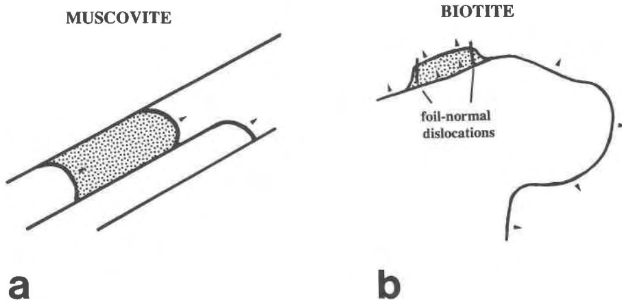
Fig. 4. Diagrams of dislocation activation observed in muscovite and biotite. Arrows indicate the direction of dislocation motion. (a) The advance of a step parallel to a dislocation line, typical of screw dislocation glide. In this illustration, the dark line has split, and an area of reversed contrast separates the advancing and the trailing dislocation. (b) The passage of a dislocation around an obstacle by dissociation.
