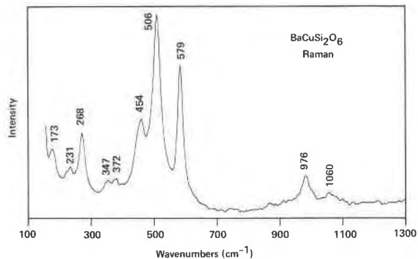
Fig. 3. Raman spectrum of BaCuSi 2 O 6 measured with 514.5-nm Ar-ion excitation. Bands at 500–600 cm -1 are assigned to oxygen breathing modes of the 4-membered tetrahedral rings and square-planar Cu (see text). The high-frequency bands at 900–1100 cm -1 are assigned to symmetric Si–O stretching vibrations; low-frequency bands arise from SiO 4 tetrahedral bending motions, bending modes of the square-planar Cu, and Ba–O stretching motions.
