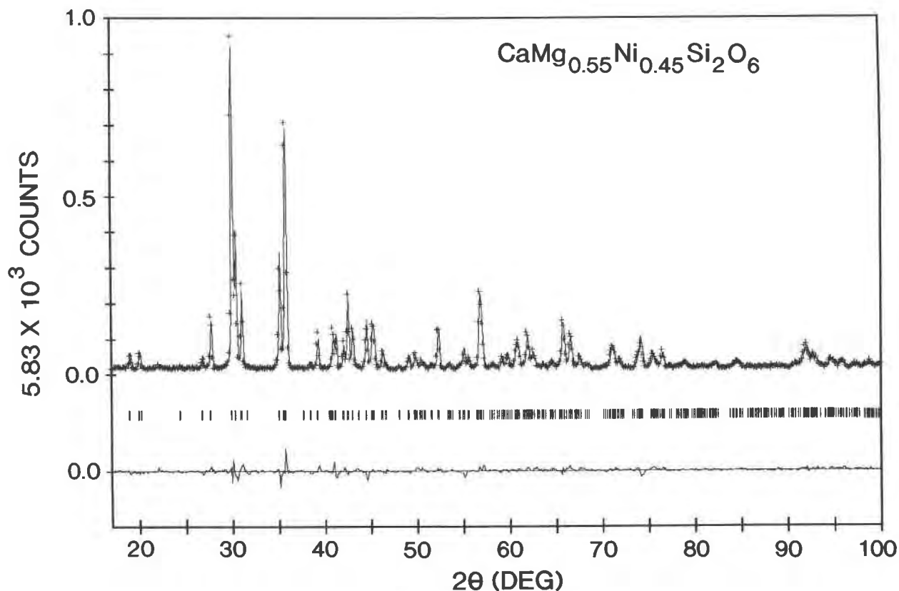
Fig. 1. Observed and calculated X-ray powder diffraction pattern for sample \text{Ni}_{50} ( \text{CaMg}_{0.55}\text{Ni}_{0.45}\text{Si}_2\text{O}_6 ). The crosses are the observed data, the solid line is the calculated pattern, and the vertical bars mark all possible Bragg reflections ( K\alpha_1 and K\alpha_2 ). The difference between the observed and calculated patterns is shown at the bottom.
