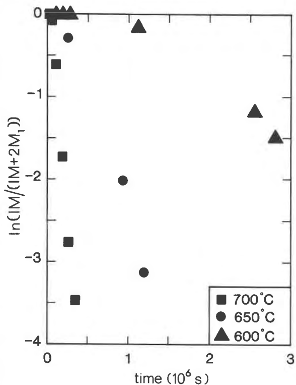
Fig. 5. Experimental data of Mukhamet-Galeyev et al. (1985) plotted as a function of \ln[1M/(1M + 2M_1)] and time ( 10^6 s) at 600, 650, and 700 °C.
