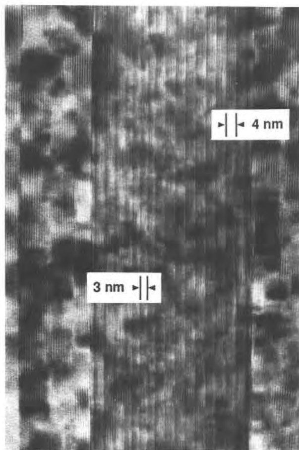
Fig. 4. The (00 l ) lattice-fringe image of illite showing ordered regions of three- and four-layer periodicity in 1M_0 from well 12, depth of 1235–1236 m.
