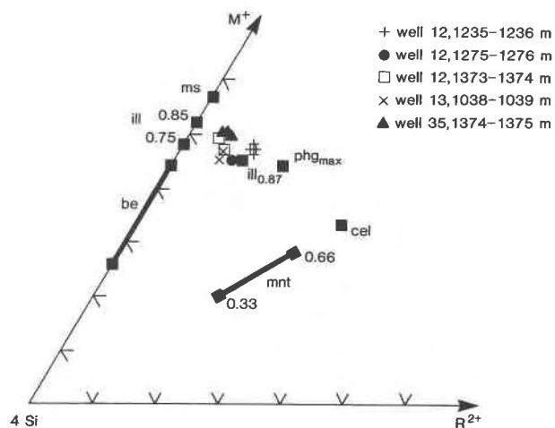
Fig. 1. Compositions of illite samples plotted on a diagram of M^{+}4Si-R^{2+} after Meunier and Velde (1989). Abbreviations are be = beidellite, cel = celadonite, ill = illite, mnt = montmorillonite, ms = muscovite, and phg_{max} = maximum phengite substitution. M^{+} is the layer charge, 4Si is the maximum Si content of the tetrahedral sheet, and R^{2+} is the total number of divalent cations in the octahedral site. Layer charges per O_{10}(OH)_2 are given by the numbers (0.33, 0.66, 0.75, 0.85, 0.87). Meunier and Velde (1989) and references therein list coordinates of the phyllosilicates in the M^{+}4Si-R^{2+} system.
