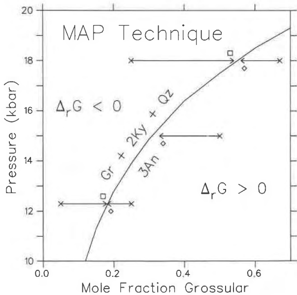
Fig. 1. Illustration of the procedure used to derive solution properties for garnet from constant temperature experiments on the displacement of the equilibrium 3\text{An} = \text{Gr} + 2\text{Ky} + \text{Qz} . Crosses and arrowheads show the starting and final garnet compositions, respectively. Uncertainties in pressure and final compositions are incorporated into the P - X_{\text{Gr}} location of constraints used in the analysis. Squares and diamonds represent inequality brackets with \Delta_r G < 0 and \Delta_r G > 0 , respectively.
