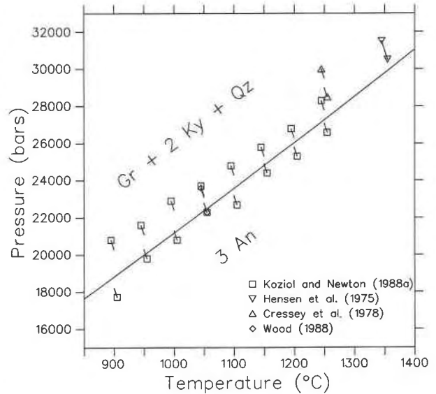
Fig. 2. Comparison of various experimental brackets for the equilibrium 3\text{An} = \text{Gr} + 2\text{Ky} + \text{Qz} with its position calculated with the thermodynamic data of Berman (1988). Open symbols represent location of experiments after adjustment of nominal values (end of lines) for estimated P - T uncertainties. The data of Koziol and Newton (1988a) and Wood (1988) have been adjusted downward by 0.2 kbar for friction effects (see text). The uncorrected data of Hensen et al. (1975) and Cressey et al. (1978) shown in this figure appear to require downward adjustment of about 1 kbar, presumably owing to friction effects.
