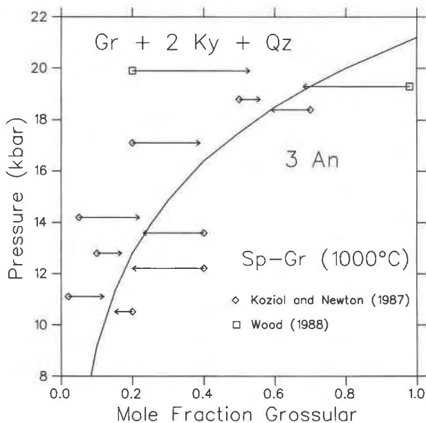
Fig. 11. Comparison of experimental brackets for the equilibrium 3An = Gr + 2Ky + Qz in the spessartine-grossular system with its position calculated assuming ideal mixing. Symbols with arrows show starting and final garnet compositions, respectively.
