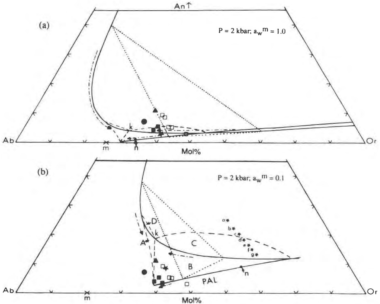
Fig. 4. Calculated phase relations in the system Ab-Or-An ( \text{H}_2\text{O} ) at 2 kbar for (a) a_w = 1.0 , and (b) a_w = 0.1 showing the plagioclase + alkali feldspar + L (PAL) curve and the corresponding polythermal solvus section (which indicates the compositions of feldspars in equilibrium with melt along the PAL curve). The calculated composition of feldspar at the consolute point on the polythermal solvus section is given by the letter k . The trachytes of Fig. 1 are plotted for reference. The arrowheads on the Ab-Or base indicate the position of the An-free thermal minimum. Selected three-phase triangles have been included for reference. (a) The composition represented by the star is from southeast Queensland (with projected composition \text{An}_{47}\text{Ab}_{38.5}\text{Or}_{14.5} ); the evolution of its melt and crystalline phases during equilibrium crystallization are shown by the dash-dot curves with arrows. The dashed field boundaries are as in (b) below; the field labels (A–D in [b]) have been omitted for clarity. (b) a_w = 0.1 .
