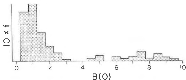
Fig. 2. A histogram of the average equivalent isotropic displacement factor for the oxygen atom, B(\text{O}) , in silica polymorphs and clathrasils.
