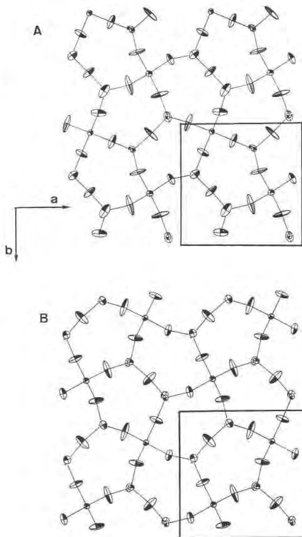
Fig. 4. ORTEP plot of the average low- \text{Ca}_2\text{ZnGe}_2\text{O}_7 structure viewed along the c axis. Note the strong anisotropy of displacement ellipsoids, which is caused by the incommensurate fine structure. (A) layer type A at z \approx 1/6 ; (B) layer type B at z \approx 1/2 . (Scale of displacement ellipsoids is 50%.)
