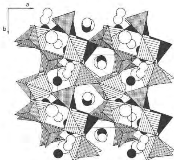
Fig. 3. Coordination polyhedron diagram of the average low- \text{Ca}_2\text{ZnGe}_2\text{O}_7 structure viewed along the c axis. Melilite-type layers are stacked in an ABA'ABA' sequence. Large open circles represent Ca atoms at z \approx 0, 1 , filled small circles Ca atoms at z \approx 1/3 , and open small circles Ca atoms at z \approx 2/3 . The peanut-shaped overlapping circles are due to split Ca atoms with the same z coordinate. For a more detailed description of the structure consult the text.
