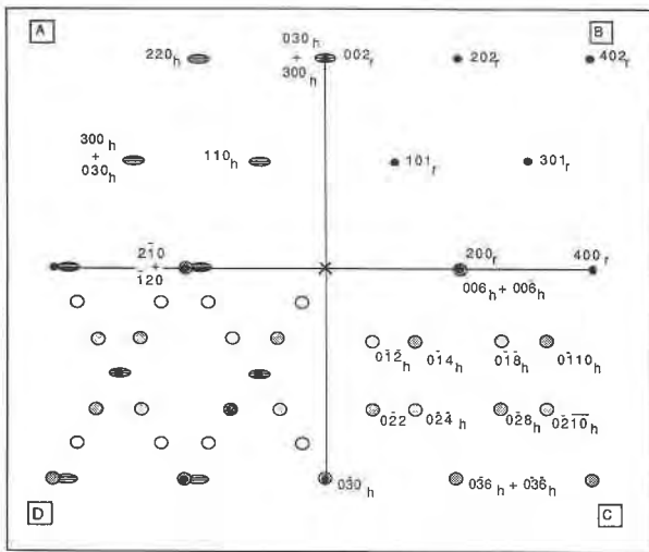
Fig. 12. Diagram illustrating the electron diffraction patterns from rutile and twinned platelets in two orientations: (a) [001] and [00 \bar{1} ] of hematite; (b) [010] of rutile; (c) [100] and [ \bar{1} 00] of hematite. The diffraction pattern resulting from the superposition of a, b, and c is illustrated in (d). Open circles indicate additional reflections resulting from dynamical diffraction.
