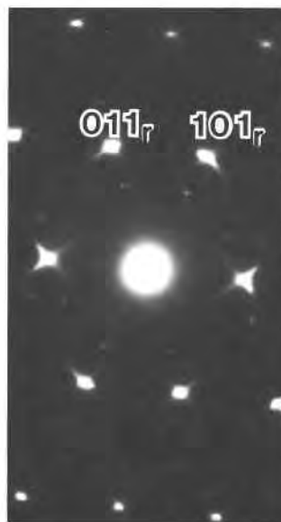
Fig. 3. SAED pattern for [111] zone from rutile (sample 2112) illustrating the presence of a superlattice with a repeat of 3 \times d_{(101)} , splitting of 1\bar{1}0 and \bar{1}10 rutile reflections, and pronounced streaking of subcell reflections.
