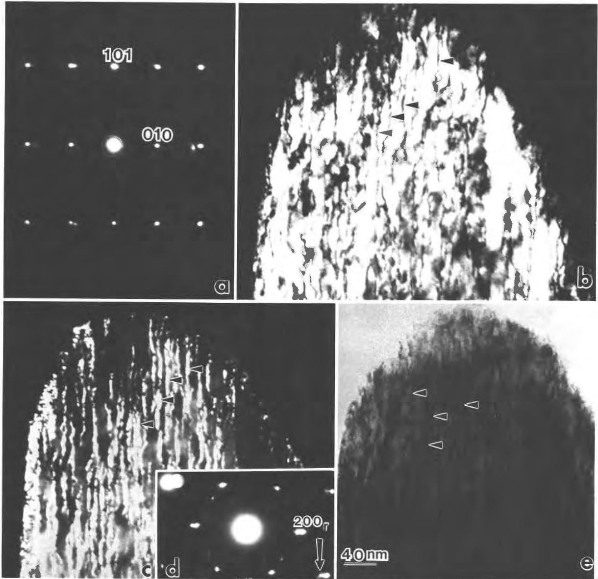
Fig. 6. (a) SAED pattern from [101] rutile (F165) showing splitting of subcell reflections; (b) dark-field image formed from rutile reflection; (c) dark-field image formed from additional reflection; (d) SAED pattern showing the reflection used to form the image in c (marked by image of an objective aperture); (e) bright-field image down [101] . Platelets are indicated by arrows.
