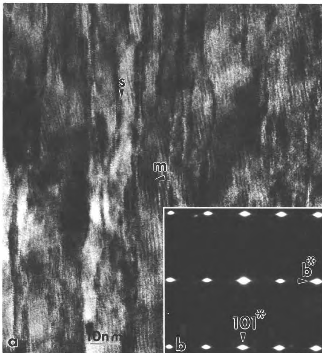
Fig. 8. (a) The [\bar{1}01] zone of rutile (sample 18) illustrating a superlattice (S) associated with the abundant lamellae. Moiré fringes (M) arise from the presence of inclined platelets; (b) corresponding SAED pattern.
