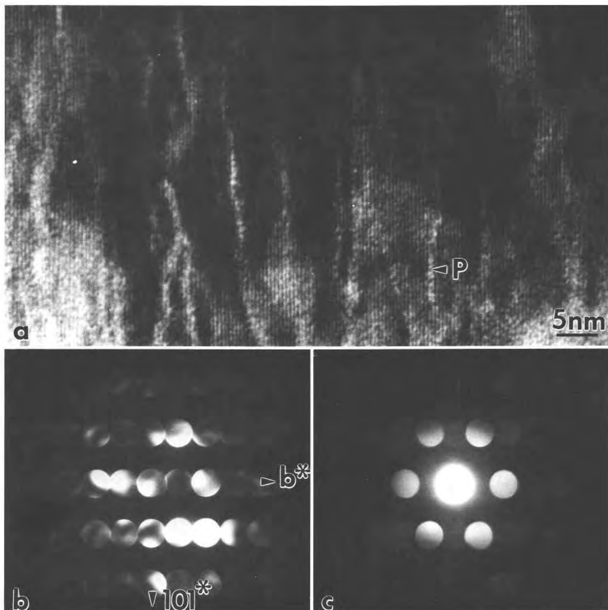
Fig. 7. (a) The [\bar{1}01] zone of rutile containing lamellae (P) parallel to (010). Micro-CBED pattern from rutile host (b) and from lamellae (c).
