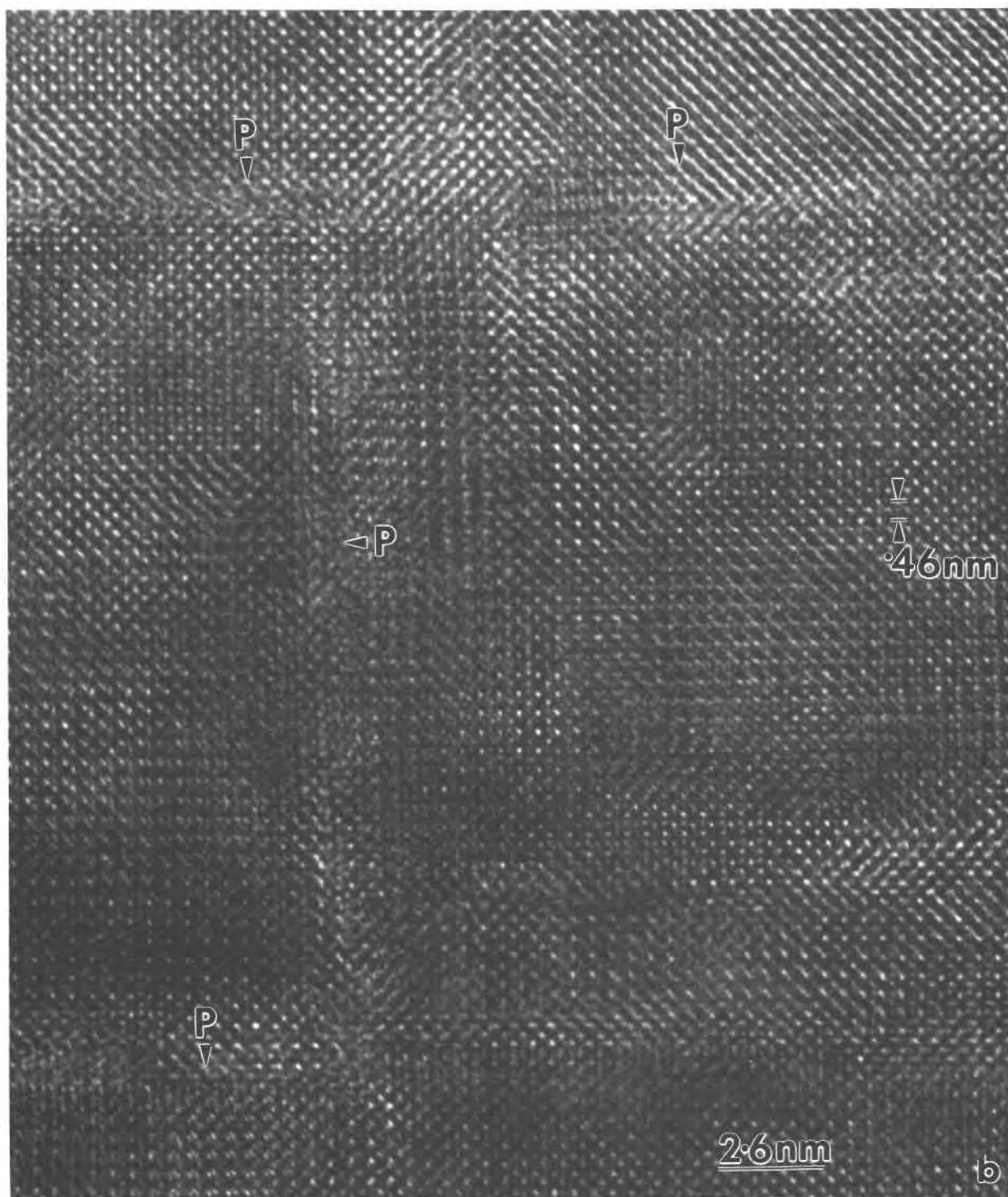
Fig. 2. (b) High-resolution images viewed down [001] of rutile (sample 2113) showing that platelets (P) are apparently \sim 1 nm wide.
