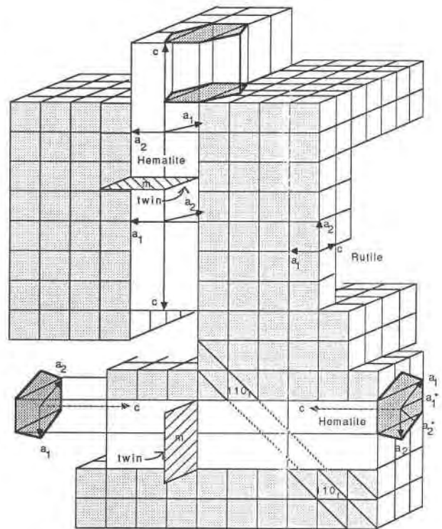
Fig. 13. Block diagram illustrating the intergrowth of twinned hematite platelets parallel to (100) and (010) of rutile. Solid lines labeled (110), and their dotted extrapolations illustrate the offset of these planes evident in Figure 2c.
