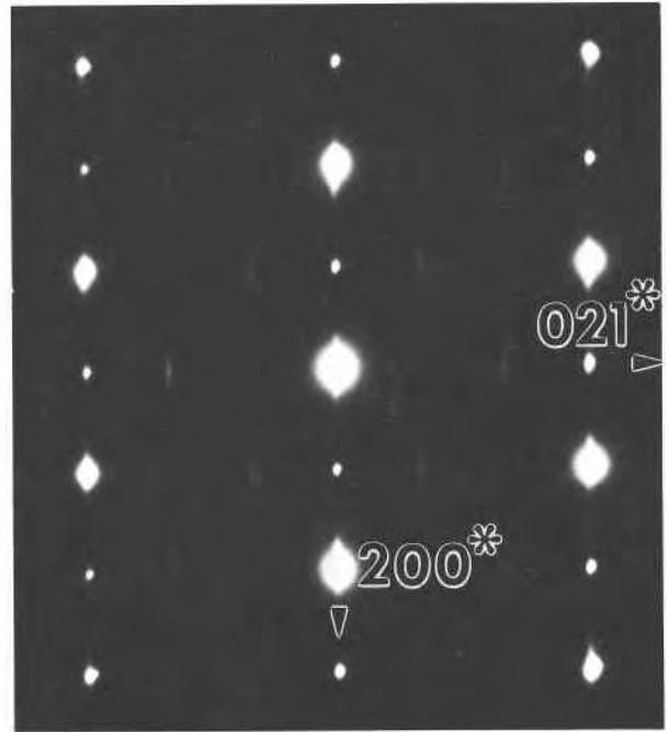
Fig. 5. SAED pattern viewed down [0\bar{1}2] (sample F165) illustrating elongate superlattice reflections.
