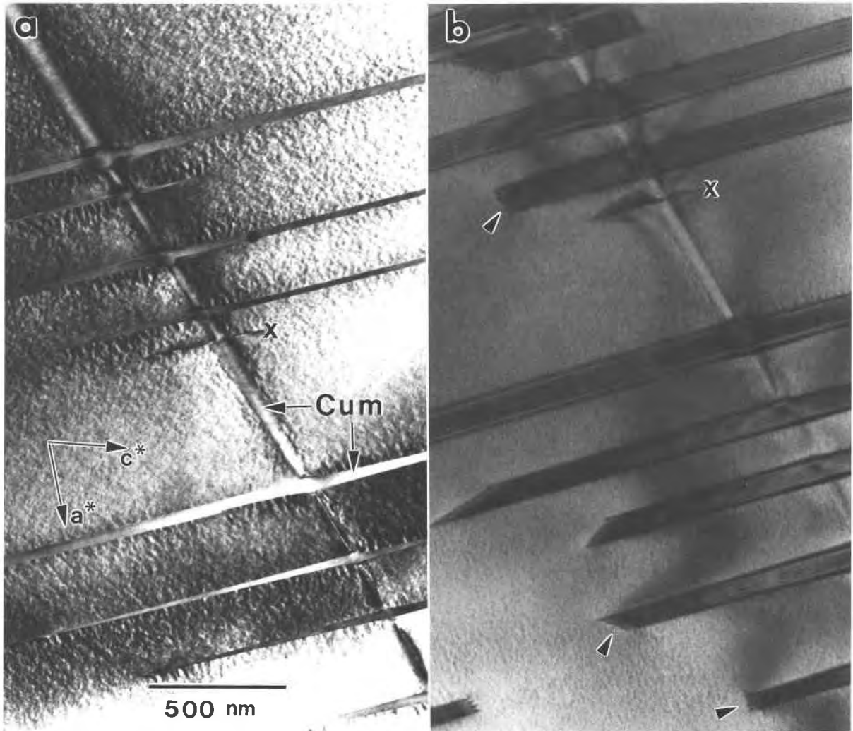
Fig. 12. (a) Bright field TEM image viewed down the b axis in a subgrain showing a single “T01” and several “100” cummingtonite lamellae. Between these large cummingtonite lamellae is pervasive fine-scale actinolite-hornblende exsolution. This texture has coarsened somewhat at cummingtonite lamellar interfaces. (b) Same area in tilted orientation. The “x” marks identical locations in parts a and b. Note the dislocations at the tips of the “100” cummingtonite lamellae (arrows).
