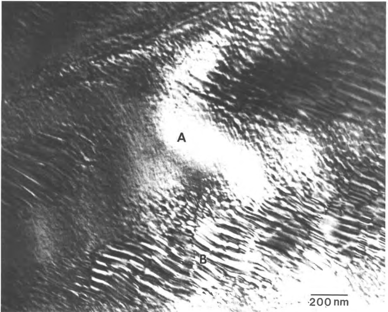
Fig. 13. Bright field TEM image of a small ( \sim 3.5 \mu\text{m}^2 ) area showing actinolite-hornblende exsolution ranging from very fine scale tweed (A) to fairly coarse tweed (B). These varying textures formed as a result of compositional zoning in the bulk amphibole. Bulk AEM analyses indicate that the fine scale tweed (A) has approximately 0.80 total Al atoms pfu, whereas the coarse tweed (B) has about 1.45 total Al atoms pfu. Note also that the lamellar interfaces are curved, suggesting a variable orientation.
