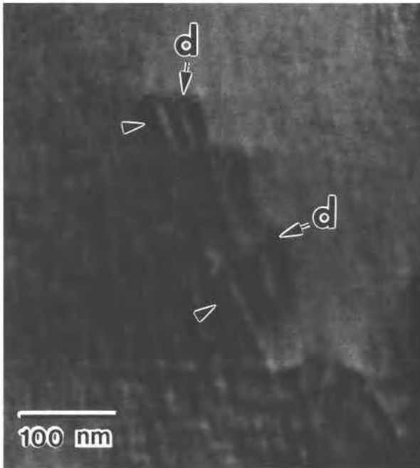
Fig. 4. Bright field TEM image of fine-scale tweed exsolution with coarsening (arrows) at dislocations (d). These dislocations may be heterogeneous nucleation sites. A nonzone-axis orientation was used to enhance contrast.
