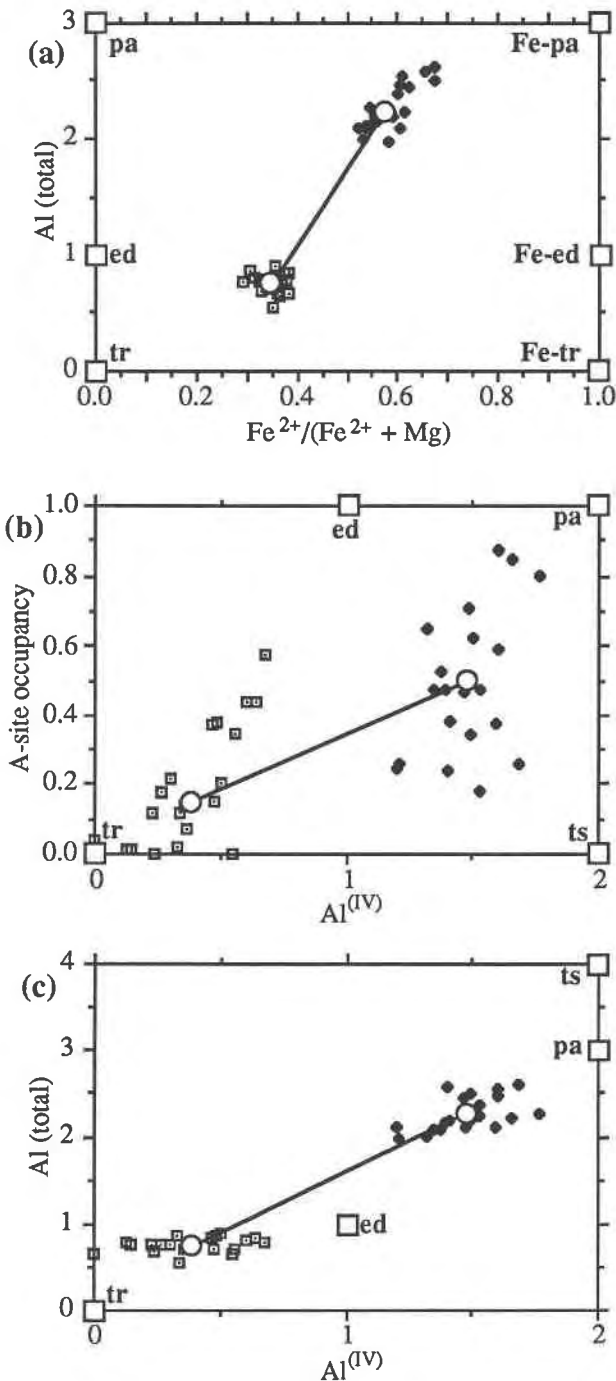
Fig. 10. Plots of AEM analyses of individual actinolite and hornblende lamellae, showing the miscibility gap. Open squares are for actinolite and filled diamonds are for hornblende. The open circles connected by a tie line represent the average compositions. (a) Plot of total Al vs. \text{Fe}^{2+}/(\text{Fe}^{2+} + \text{Mg}) . (b) Plot of calculated A-site occupancy vs. ^{14}\text{Al} . (c) Plot of \text{Al}_{\text{tot}} vs. ^{14}\text{Al} . Abbreviations for end-members as in Figure 8.
