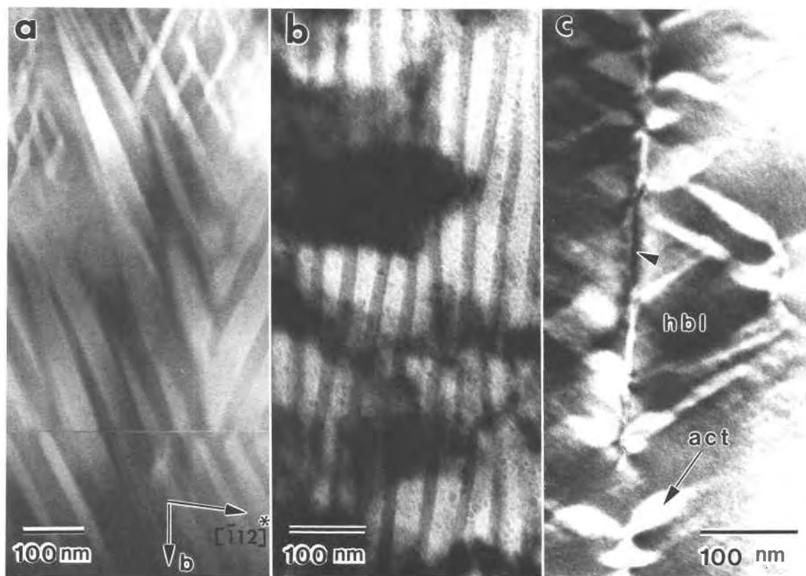
Fig. 9. Bright field TEM images of anomalously coarse exsolution textures where AEM analyses of individual lamellae were obtained. (a) Coarse exsolution viewed down [201] zone. This is a lower magnification image of the area shown in Figure 7a. The sharp horizontal feature near the bottom is a chain-width error. (b) In this nonzone-axis orientation one set of lamellae, running north to south, has short dimensions nearly parallel to the plane
