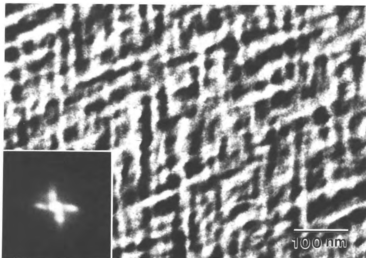
Fig. 6. TEM image of coarse tweed texture tilted so that both sets of compositional modulations are in strong diffracting orientation. The inset shows a greatly enlarged diffraction spot surrounded by satellite reflections, indicating the periodic nature of the microstructure. This observation is suggestive of spinodal decomposition.
