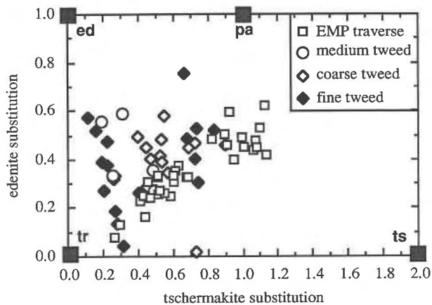
Fig. 8. Plot of EMP and AEM bulk amphibole compositions from porphyroclasts and subgrains in terms of tschermakite and edenite substitution vectors. These compositions cover much of the calcic amphibole series and span the actinolite-hornblende solvus. The scatter in the edenite component for the AEM analyses probably results from analytical errors for Na, as discussed in the text. End-members are tr = tremolite, ed = edenite, pa = pargasite, ts = tschermakite.
