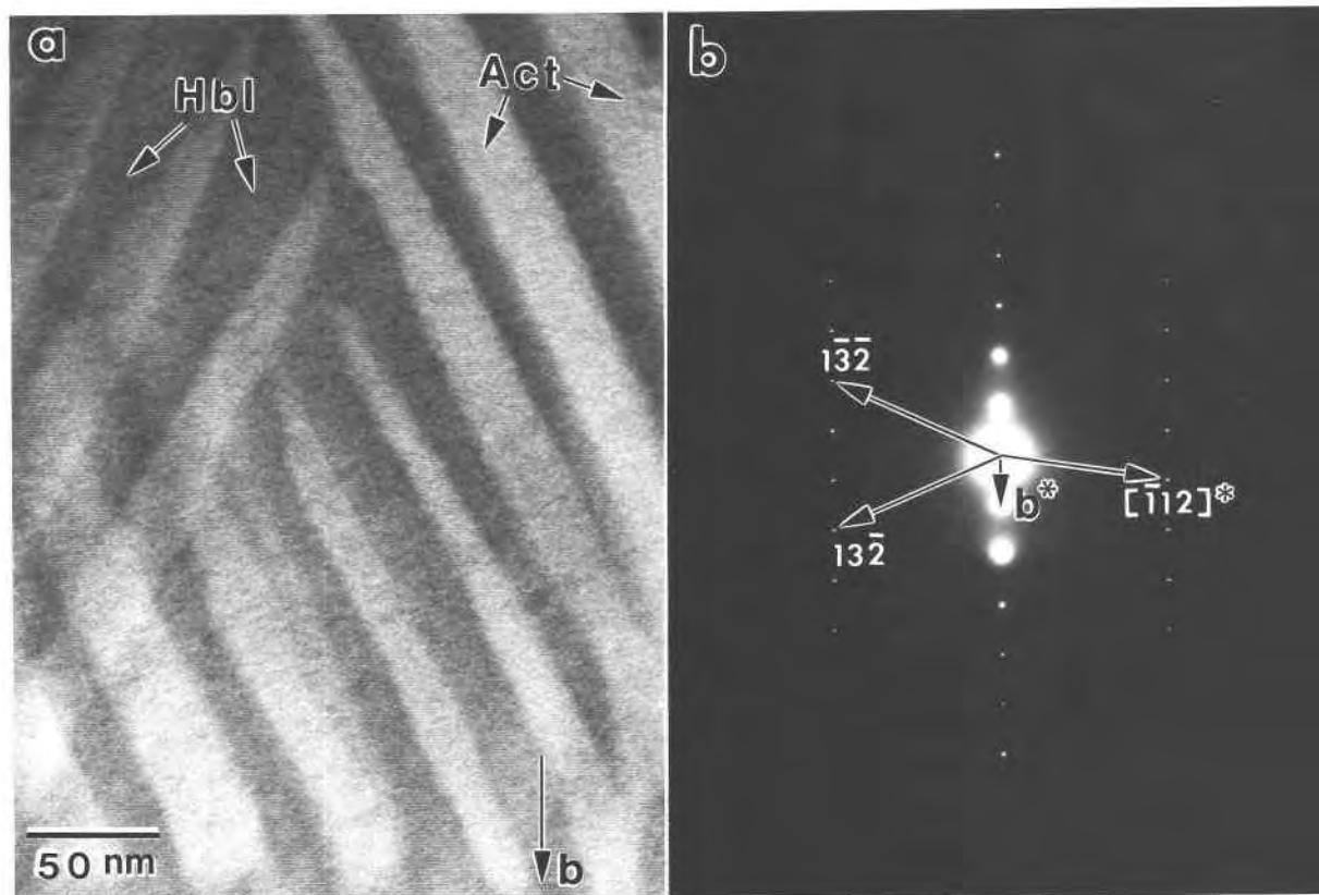
Fig. 7. Orientation of actinolite-hornblende exsolution lamellae. (a) TEM image viewed down [201] of an anomalously coarse area. Note that the lamellar interfaces are relatively straight and sharp. (b) Corresponding SAED pattern of the [201] zone, showing the b^*-[112]^* reciprocal lattice plane. The 132 and 132 reflections have been labeled in the diffraction pattern. Note that the [132]^* reciprocal lattice vector is nearly perpendicular to the
