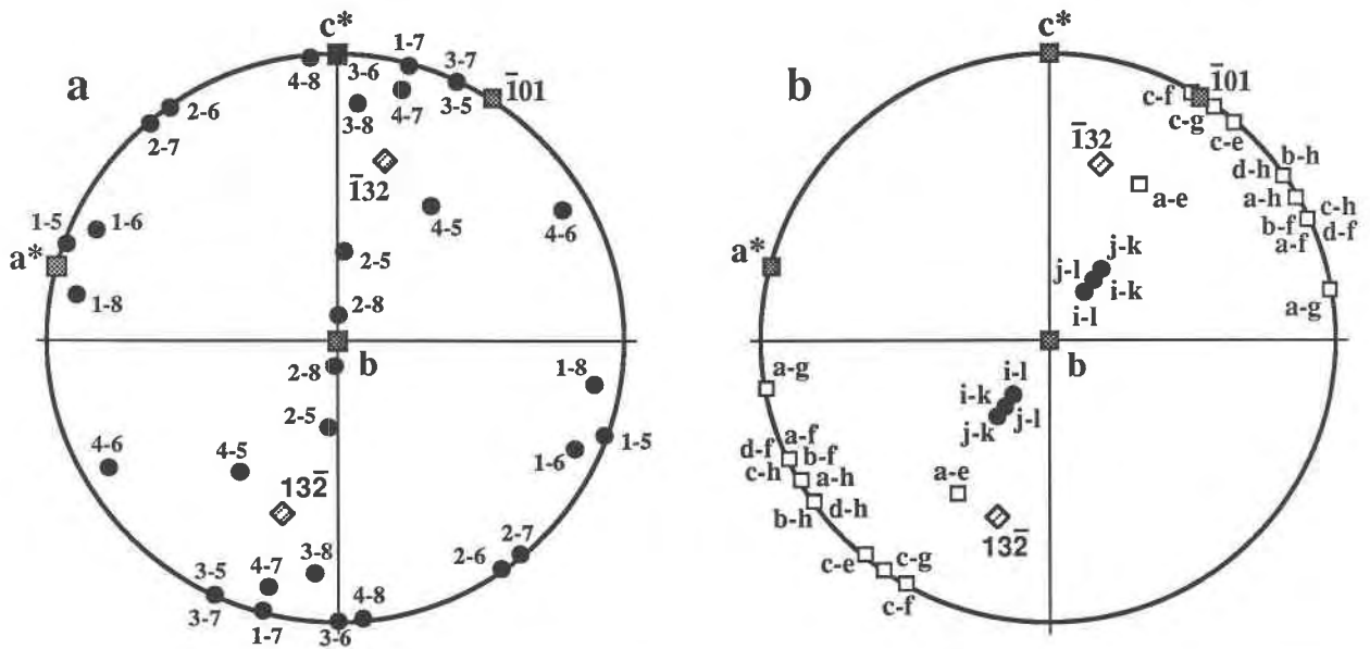
Fig. 11. Stereographic projections down b showing results from EPLAG calculations for intergrown actinolite-hornblende. Poles for (001), (010), (100), and (\bar{1}01) are shown as stippled boxes. The observed orientations, " 13\bar{2} " and " \bar{1}32 ," are shown as diamonds. (a) Numbered filled circles are poles to optimal phase boundaries calculated using literature unit cells shown in Table 9 (see cells 1 through 8). Actinolite-hornblende pairs are labeled on the stereogram. Note that pairs 3-8, 4-5, and 4-7 are fairly near the observed orientation. (b) Open squares are poles to optimal phase boundaries calculated using the model unit-cell
