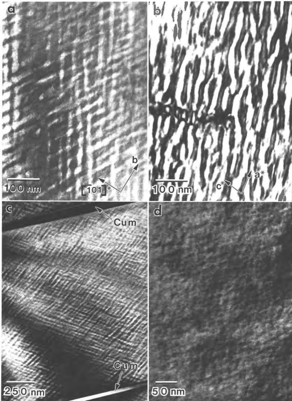
Fig. 2. Bright field TEM images of pervasively twinned exsolution textures in complex calcic amphiboles (a) Coarse twinned texture in a large porphyroblast viewed down [101] . Note that the compositional modulations occur in two symmetrical orientations. (b) Coarse twinned in a subgrain viewed parallel to b . The lamellar interfaces appear curved in this highly tilted orientation. (c) Pervasive twinned exsolution with two larger, “100” cummingtonite lamellae. This area is tilted out of a zone-axis orientation. (d) Fine-scale twinned texture in an actinolitic subgrain, which probably represents the initial stages of spinodal decomposition. Electron beam is parallel to [101] .
