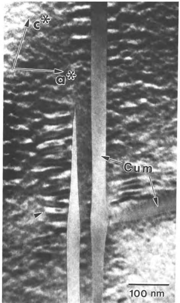
Fig. 5. Bright field TEM image showing coarsening (arrow) of tweed exsolution at “100” cummingtonite lamellar interfaces. The electron beam is parallel to b . Coarsening may have been enhanced because of the strain energy at these interfaces, or these may be sites of heterogeneous nucleation.
