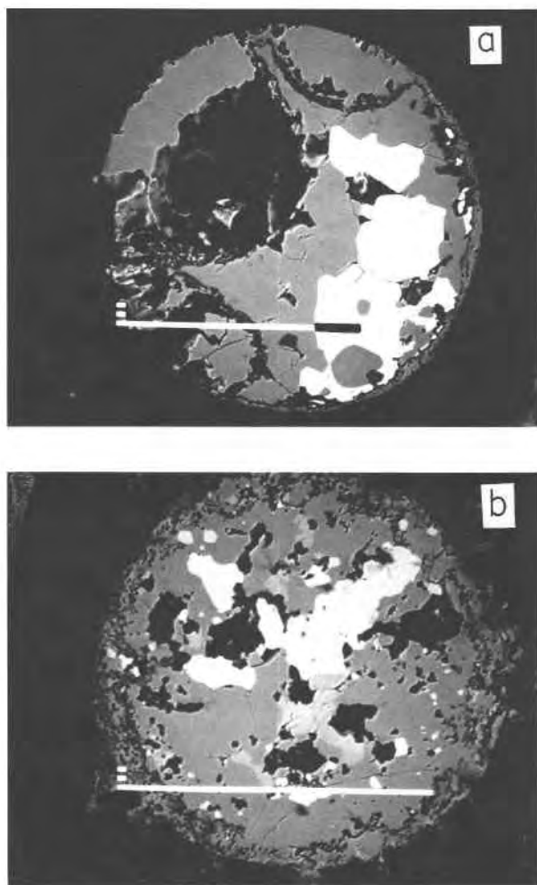
Fig. 2. Backscattered electron images of two additional opaque nodules in chondrule 90-1. Rounded to anhedral awaruite grains (white in a and b) are surrounded by magnetite (dark gray). The nodule in (b) contains some pentlandite (medium gray). Black areas are plucked regions. In both images, the scale bar is 100 \mu\text{m} long; in (a), the portion of the scale bar overlapping an awaruite grain is black.
