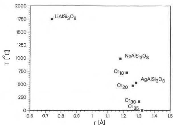
Fig. 4. Temperature of the triclinic/monoclinic transformation in disordered feldspars \text{MAISi}_3\text{O}_8 as a function of cation radius (for observed coordination). Data for sanidine-analbite series from Kroll (1984).
