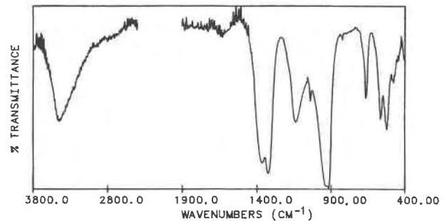
Fig. 3. Infrared spectrum of ashburtonite.
