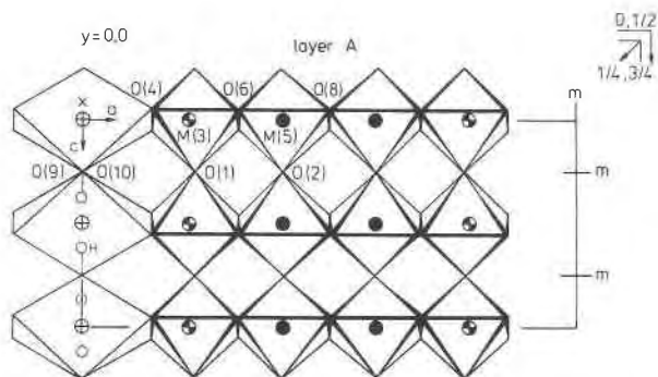
Fig. 1. Projection parallel to [010] of the A layer in kornerupine at y = 0 .
