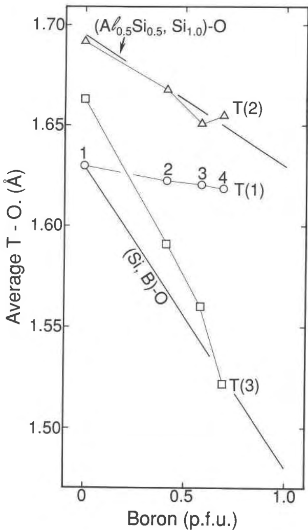
Fig. 5. Average tetrahedral distances are plotted as a function of B content (in atoms B per formula unit from chemical analysis) of the four kornerupine samples for which the crystal structure has been refined. Lines join average ^{14}\text{Si}-\text{O} = 1.63 \text{ \AA} and ^{10}\text{B}-\text{O} = 1.48 \text{ \AA} and average ^{14}\text{Si}-\text{O} and ^{14}(\text{Al}_{0.5}\text{Si}_{0.5})-\text{O} = 1.695 \text{ \AA} calculated for an average O coordination of 3.5 from data of Shannon (1976). Sources of chemical and crystallographic data are as follows: (1) B = 0, Limpopo Belt, southern Africa, Grew et al. (1990), this paper; (2) B = 0.41, Mautia Hill, Tanzania, McKie (1965), Moore et al. (1989); (3) B = 0.58, synthetic, Werdinger and Schreyer (1978), Moore and Araki (1979); and (4) B = 0.69, Grenville Province, Canada, Finger and Hazen (1981).
