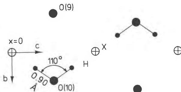
Fig. 4. Projection parallel to [100] of the H and O positions in the vicinity of the X site at x = 0 .
