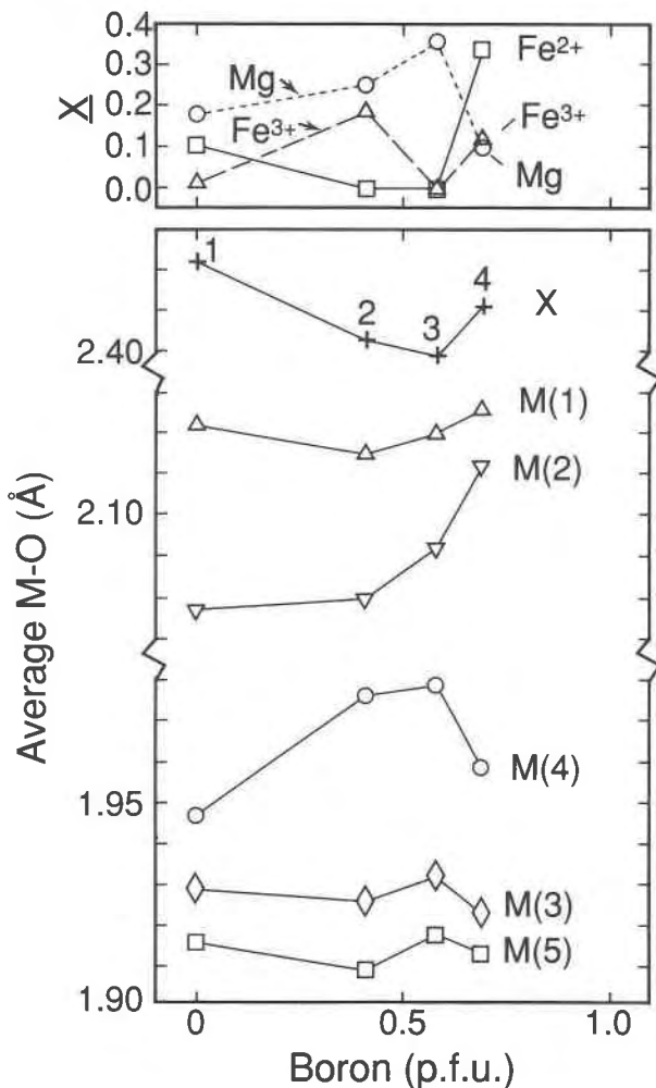
Fig. 6. Average octahedral and X-site distances are plotted as a function of B content (in atoms B per formula unit from chemical analysis) of the four kornerupine samples for which the crystal structure has been refined (sources of data are given in Fig. 5). The following mole fractions X are plotted: X_{\text{Fe}^{2+}} = \text{Fe}^{2+}/(\text{Fe}^{2+} + \text{Mg}) in M1, M2, and X (solid line), X_{\text{Fe}^{3+}} = \text{Fe}^{3+}/(\text{Fe}^{3+} + \text{Mg} + \text{Al}) in M4 (long-dashed line), and X_{\text{Mg}} = \text{Mg}/(\text{Fe}^{3+} + \text{Mg} + \text{Al}) in M4 (short-dashed line). The mole fractions were calculated from the chemical analyses and site occupancies; X_{\text{Mg}} in no. 3 was calculated from the average M4-O distance, assuming \text{Al-O} = 1.91 \text{ \AA} and \text{Mg-O} = 2.10 \text{ \AA} (see Moore et al., 1989).
