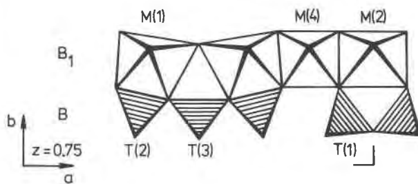
Fig. 3. Projection parallel to [001] of a portion of the kornerupine structure at z = 0.75 .
