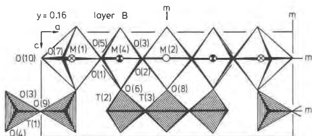
Fig. 2. Projection parallel to [010] of the B layer in kornerupine at y = 0.16 .
