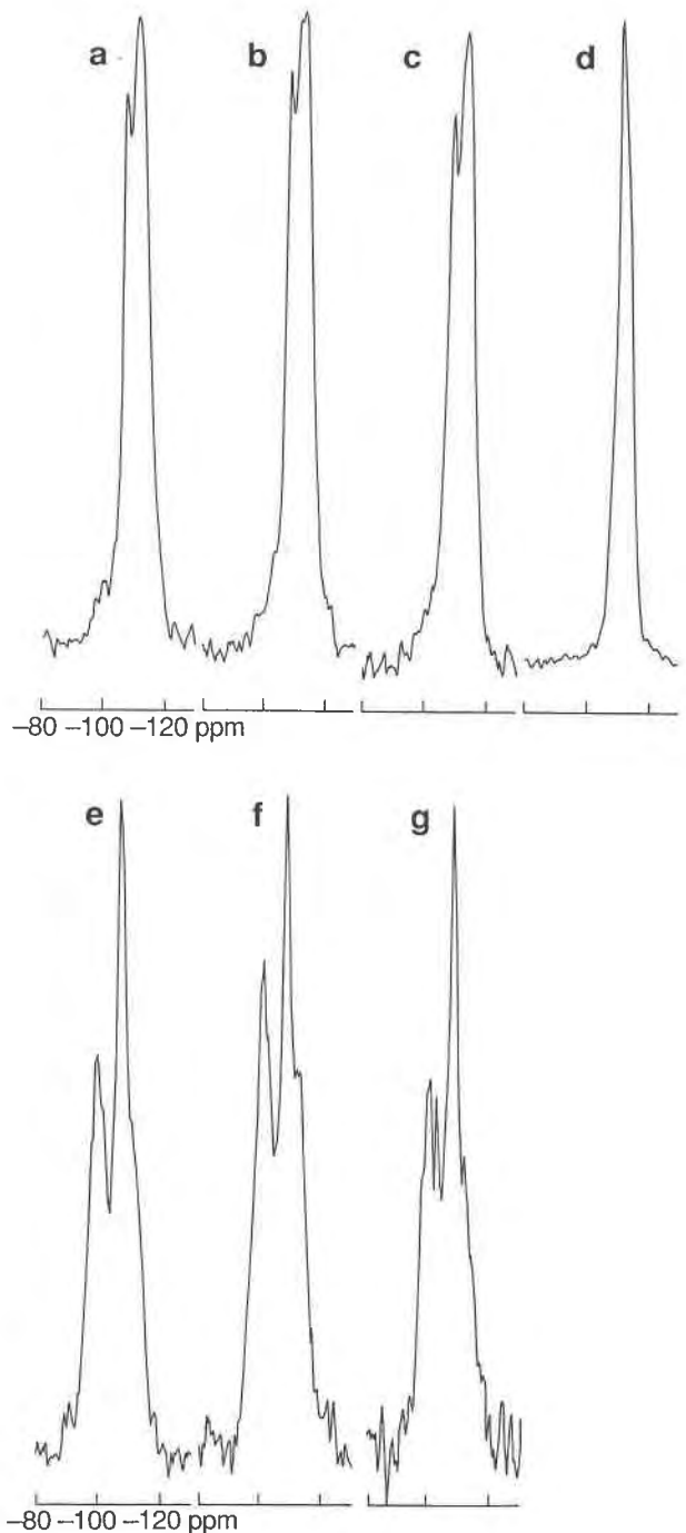
Fig. 4. Spectra of ^{29}\text{Si} MAS-NMR of wood opal (S11); a-d = with MAS only and e-g = with CP-MAS and 10-ms contact time. a and e before heat treatment, b and f after heating at 160^\circ\text{C} for 8 h, c and g after heating at 360^\circ\text{C} for 8 h, and d after heating at 1150^\circ\text{C} for 8 h.
