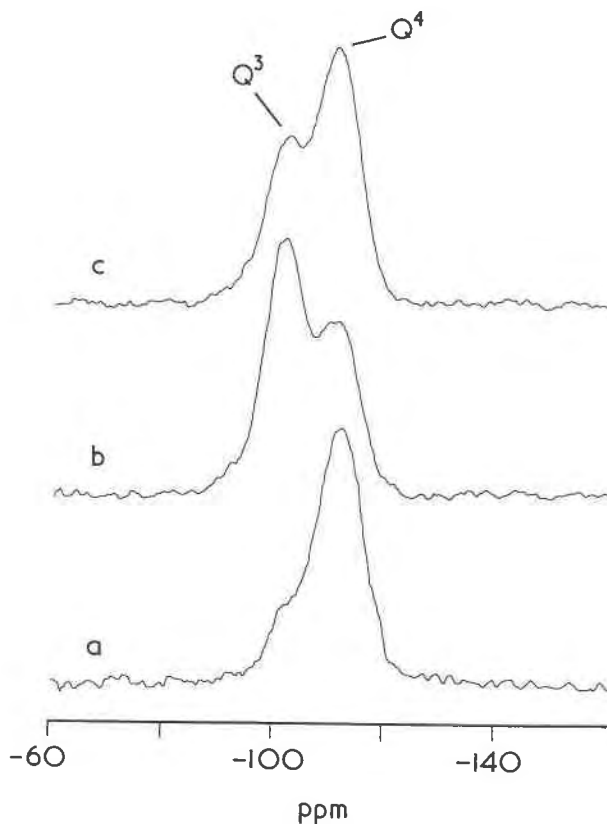
Fig. 3. Spectra of ^{29}\text{Si} NMR (MSL-300) of opal sample S27; a = with MAS and high power ^1\text{H} decoupling, b = with MAS + decoupling + CP with 1-ms contact time, and c = with MAS + decoupling + CP with 4-ms contact time.
