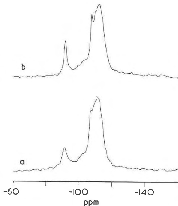
Fig. 2. Spectra of ^{29}\text{Si} MAS-NMR (MSL-300) of Beltane opal (S3); a = with MAS only and b = with both MAS and high power ^1\text{H} decoupling.
