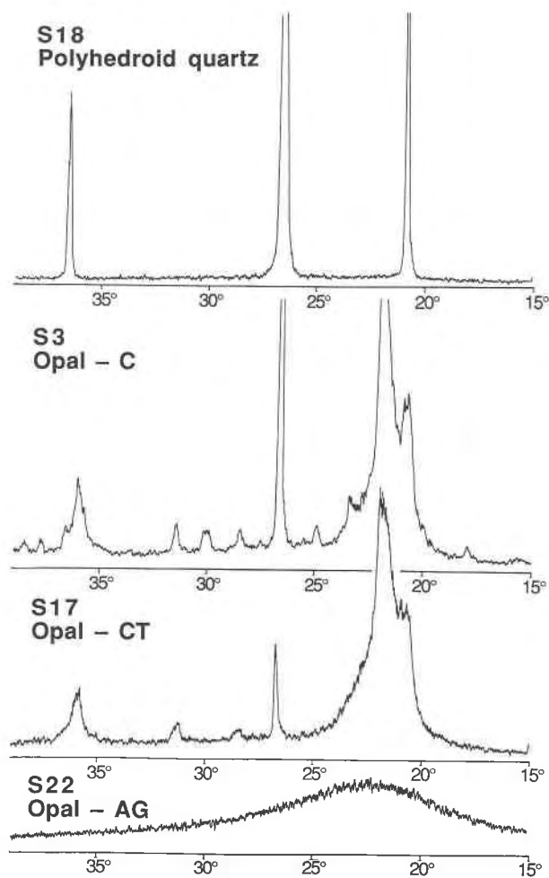
Fig. 1. X-ray powder diffraction patterns of opal-AG (S22), opal-CT (S17), opal-C (S3), and polyhedroid quartz (S18).
