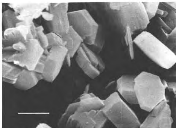
Fig. 2. SEM photograph of boromuscovite from the NAP showing euhedral pseudohexagonal flakes. Scale bar equals 2 \mu\text{m} .
