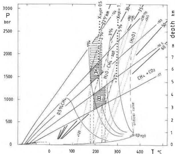
Fig. 6. The estimation of fluid trapping P - T conditions from isochores. The isochores for the CH 4 -CO 2 inclusions (solid lines) are calculated from the Peng-Robinson equation of state (Herskowitz and Kisch, 1984); isochores for pure H 2 O (dotted lines) are taken from Fisher (1976). The assumption of CH 4 saturated H 2 O at trapping implies forming temperatures equal to T_{h, aq} (dashed lines). The isochores for the aqueous inclusions containing CH 4 (H 2 O-CH 4 -sat.) are shifted to lower temperatures compared to the isochores for pure H 2 O with the same molar volume. The estimated trapping pressures for the Silurian-Devonian of the Delaware Water Gap area (A) are significantly higher than for the anthracite region of east Pennsylvania (B). The saturation curves for 5, 3, 2, 1, and 0.5% CH 4 are extrapolated after the data of Price (1979). Also shown are the geothermal gradients corresponding to A (22 and 30 °C/km) and B (50 and 60 °C/km). The heavily dotted lines show the equilibrium of the reaction kaolinite + quartz = pyrophyllite + H 2 O at X_{H_2O} = 1 and X_{H_2O} = 0.5 .
