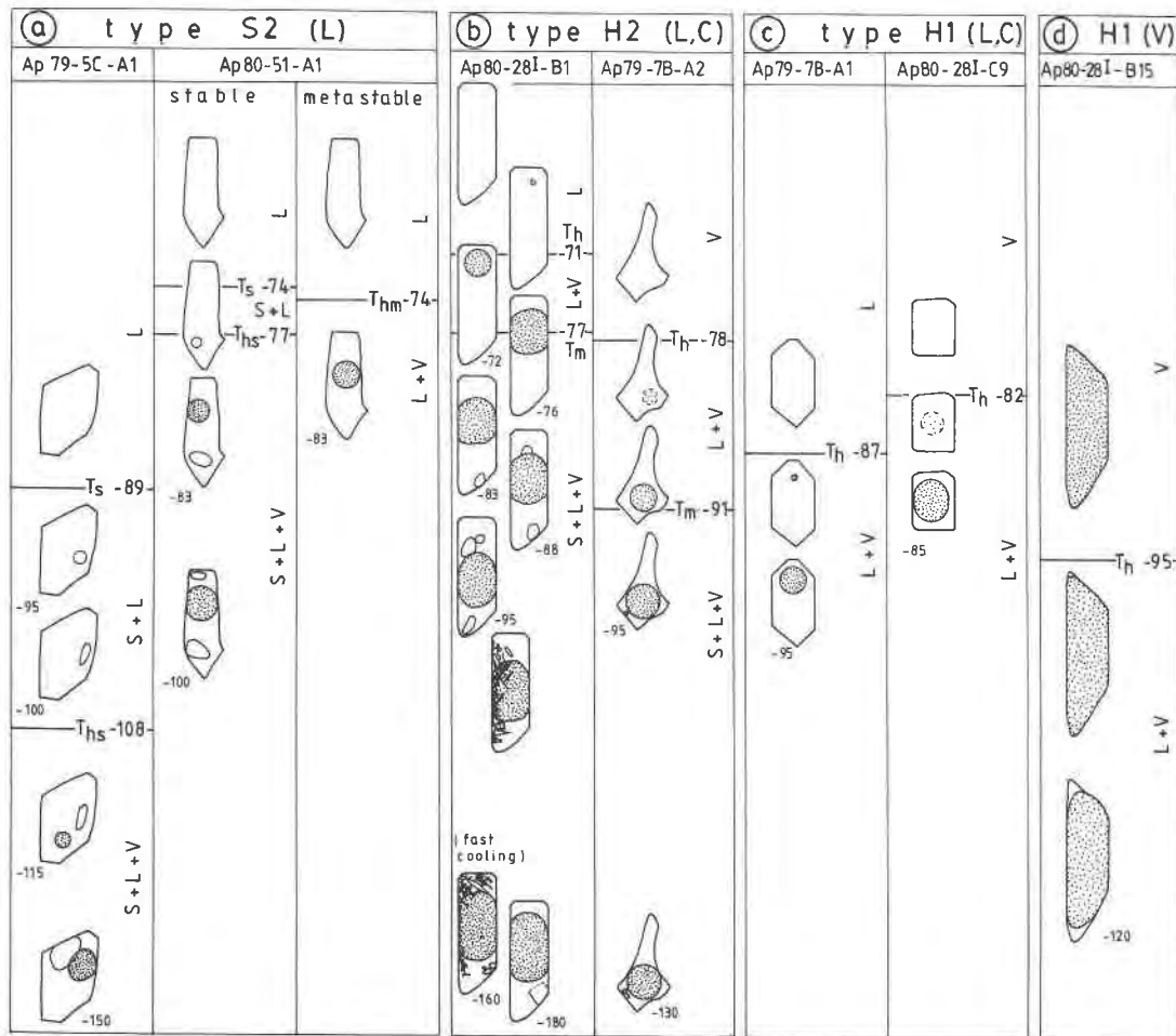
Fig. 3. Examples of phase sequences in CH 4 -CO 2 inclusions observed in the temperature range from -160 to +35 °C. The stippled parts indicate the vapor phase. (a) Type S2(L) showing the phase sequence S + L + V → S + L → L for the stable phases and L + V → L for the metastable phases. The latter transition can only be observed for inclusions that show the nucleation of the bubble before the nucleation of solid CO 2 on cooling. (b) Type H2(L) characterized by the phase sequence S + L + V →
