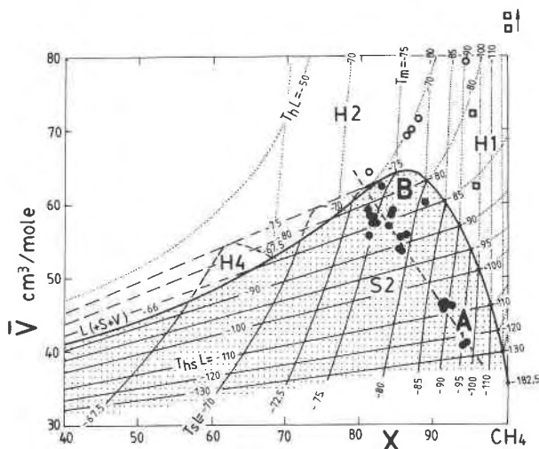
Fig. 5. \bar{V}X diagram of the system CO 2 -CH 4 for molar volumes between 30 and 80 cm 3 /mol (after Herskowitz and Kisch, 1984). The three-phase curve L(+ S + V) delimits the regions characterized by sublimation (stippled) and homogenization (open) (see text). A selection of isotherms (°C) marking partial homogenization ( T_{hL} ) and sublimation (CO 2 dissolution) ( T_{sL} ) temperatures is shown for the S-type inclusions; the isotherms marking homogenization ( T_{hL} ) and melting ( T_m ) for the H-type inclusions are tentative. Plotted are the microthermometry data of the type S2 inclusions (black dots), some H2 (open dots) and H1 inclusions (squares) from the Silurian-Devonian of the Delaware Water Gap area (A) and from the anthracite region of east Pennsylvania (B).
