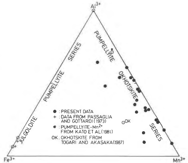
Fig. 4. Composition of Mn-rich pumpellyites and okhotskites in Al 3+ -Fe 3+ -Mn 3+ space.
