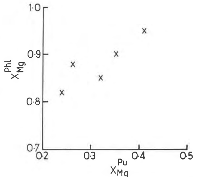
Fig. 5. Plot of X Mg Phl [= Mg/(Mg + Mn 2+ )] vs. X Mg Pu [= Mg/(Mg + Mn 2+ )]. Data from Tables 1 and 2 and unpublished source.
