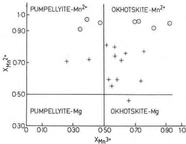
Fig. 2. Compositional plots of the pumpellyites studied in X_{Mn^{3+}} = Mn^{3+}/(Mn^{3+} + Fe^{3+} + Al) - X_{Mn^{2+}} = Mn^{2+}/(Mn^{2+} + Mg) space showing the fields of pumpellyite-(Mg), pumpellyite-(Mn 2+ ), magnesian okhotskite, designated okhotskite-(Mg), and manganese okhotskite, designated okhotskite-(Mn 2+ ) [following Passaglia and Gottardi (1973) and Kato et al. (1981); note that okhotskite-(Mg) and okhotskite-(Mn 2+ ), although following from nomenclature approved by the IMA Commission, have themselves not been approved]. Pumpellyite from type 1 assemblage = circle, pumpellyite from type 2 assemblage = plus sign.
