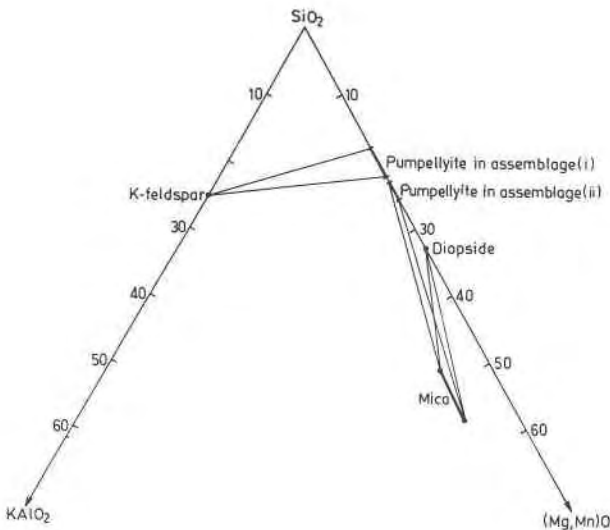
Fig. 3. Compositional plots of pumpellyites in Assemblages 1 and 2, diopside, mica, and potassium feldspar on SiO 2 -KAlO 2 -(Mg,Mn)O plane projected from braunite and calcite.
