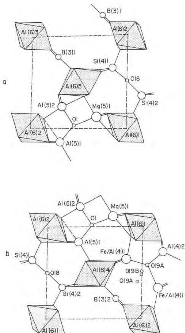
Fig. 3. Two mullite-like constituent slabs of the werdingite unit cell, each bounded by Al octahedra in the corner chains, and containing four of the 16 bridging cation sites. (a) \text{Al}_2[\text{MgAlBSi}]\text{O}_5 slab. (b) \text{Al}_2[\text{Al}(\text{Al,Fe})\text{BSi}]\text{O}_5 slab. The long fifth bond to Al(5)1 is shown by a dashed line. In the adjacent slab to the right, B in B(3)2 has been replaced by Al in Al(4)2.
