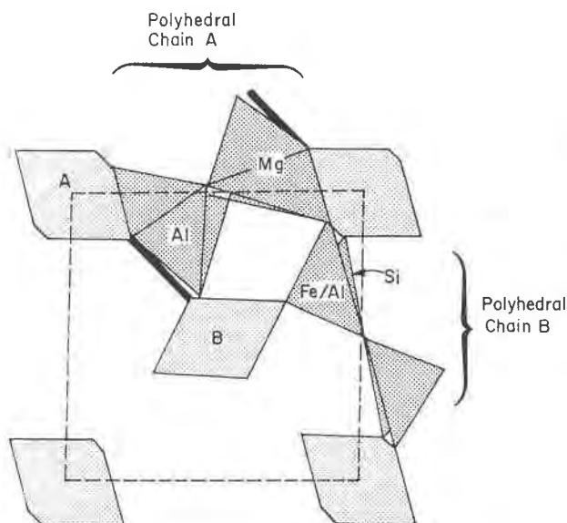
Fig. 1. Plan view of part of the werdingite unit cell, projected down [001], showing the arrangement of octahedral \text{AlO}_6 chains (dark shading) and double chains of bridging polyhedra (stippled). Vertical \text{BO}_3 triangles shown as dark solid bars.
