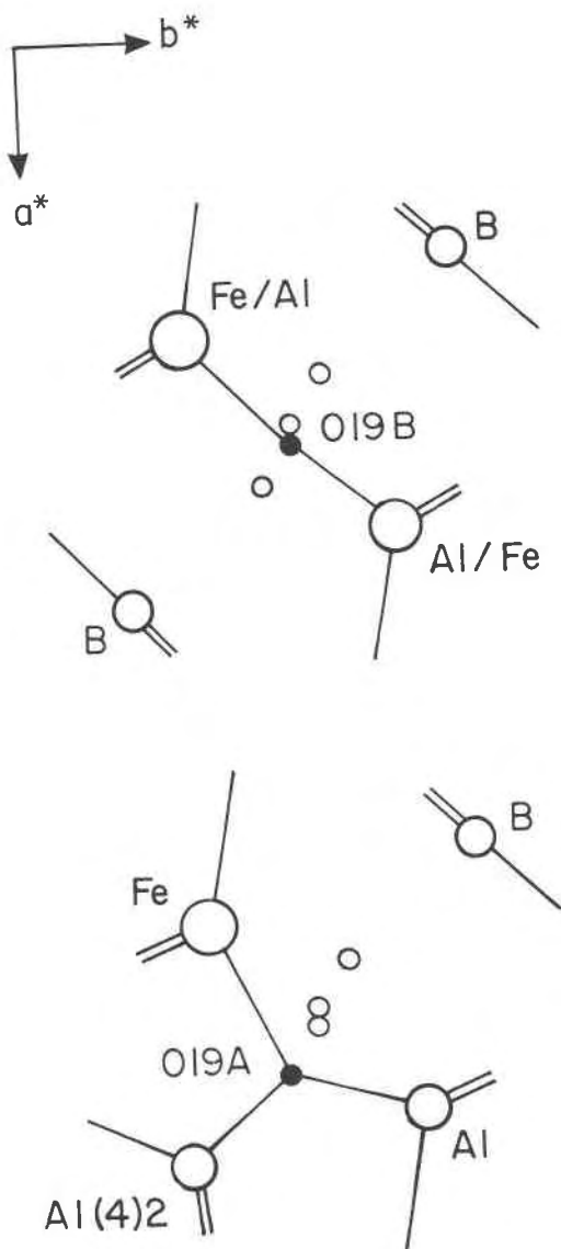
Fig. 6. Two possible configurations of cation and O site occupancy around the O19A and O19B sites in slab 2 of the werdingite structure, resulting from the substitution ^{IV}Al \rightarrow ^{III}B , viewed down [001]. Two further configurations involving the upper O19A and O19B positions are symmetrically related to these.
