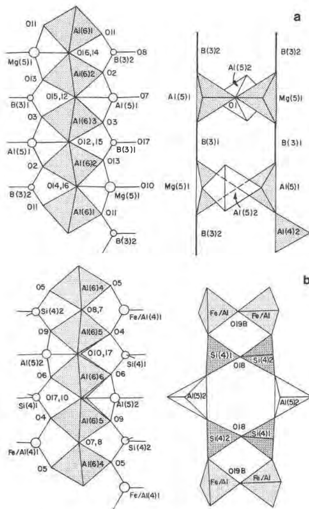
Fig. 2. Werdingite octahedral and polyhedral double chains, viewed normal to [001]. (a) Octahedral and polyhedral B-Mg-Al chains labeled A in Figure 1. (b) Octahedral and polyhedral Al/Fe-Si chains labeled B in Figure 1. Octahedral chains are viewed along the shared octahedral edges. Bridging chains are viewed normal to the plane containing the cations. \text{BO}_3 triangles appear as dark solid bars.
