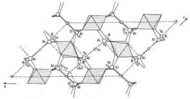
Fig. 8. A possible structure for Al_6[Al_8(B,Al)_4Si_4]O_{38} , the Mg-free B-rich mullite of Werding and Schreyer (1984), based on repetitions of werdingite slab 2.
