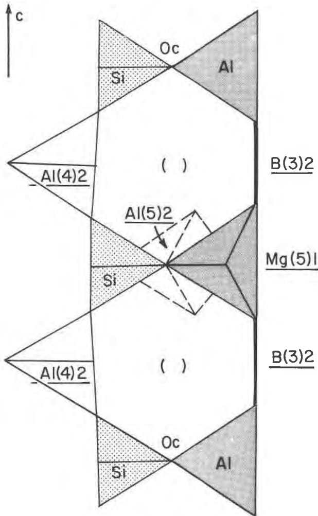
Fig. 7. A model for B substitution in sillimanite, in which an Al-Si tetrahedral double chain incorporates a werdingite-like section, with bridging O atoms O_c removed. B triangles are viewed edgewise. Parentheses mark the positions of vacant O sites, and underlined labels denote sites equivalent to those in werdingite (see Fig. 2a).
