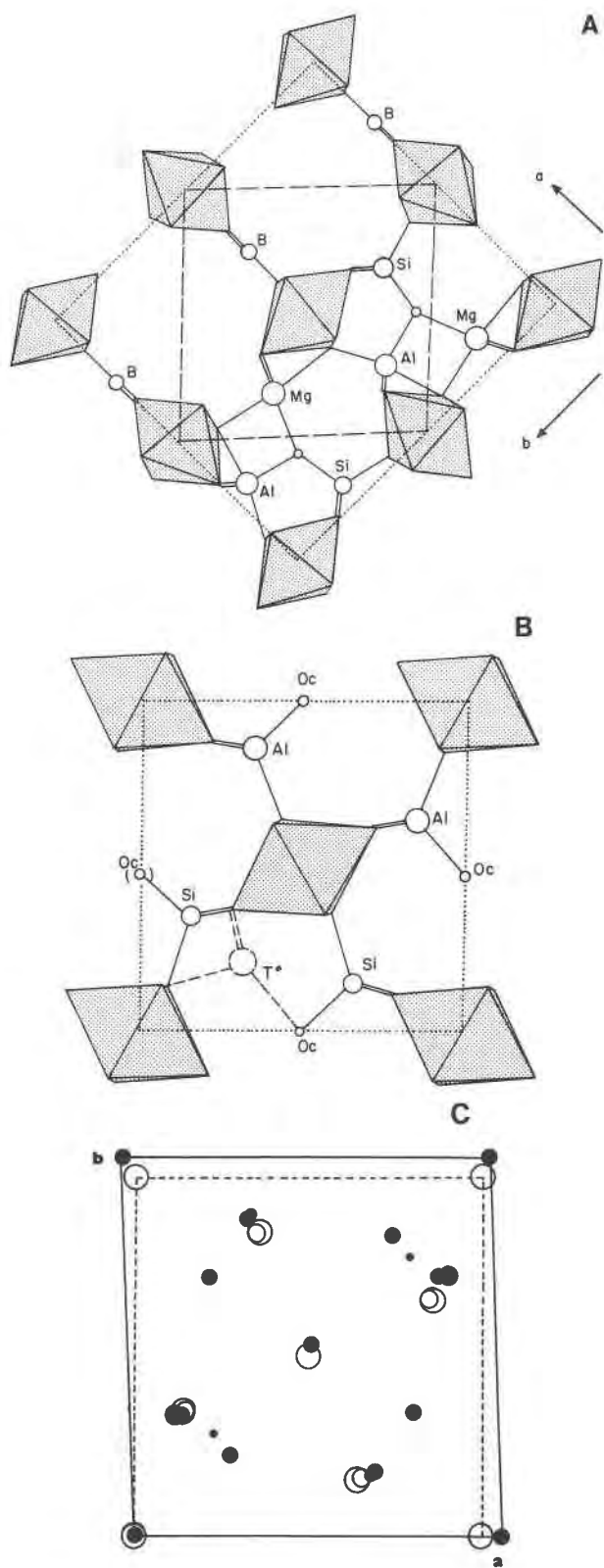
Fig. 5. Octahedral chain aluminosilicate structures related to werdingite. (A) View down [001] of lower half of the unit cell of grandidierite, after Stephenson and Moore (1968), reoriented for
