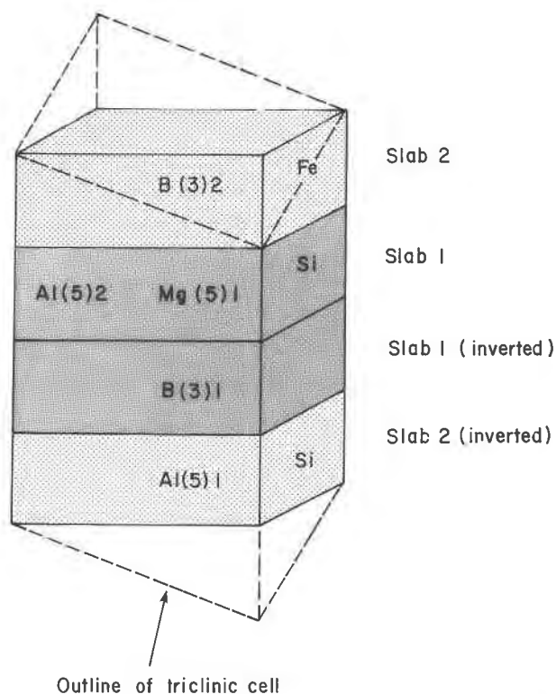
Fig. 4. Relationship of the triclinic unit cell (dashed outline) to the mullite-like slabs shown in Figure 3.
