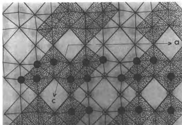
Fig. 12. Phase grating output from the SHRLI programs showing the projected positions of columns of Ti (large gray spots) and O atoms (smaller gray spots). Filled circles emphasizing the positions of the Ti atoms, open circles emphasizing the positions of the O atoms. Coordination polyhedra and axes are superimposed.
