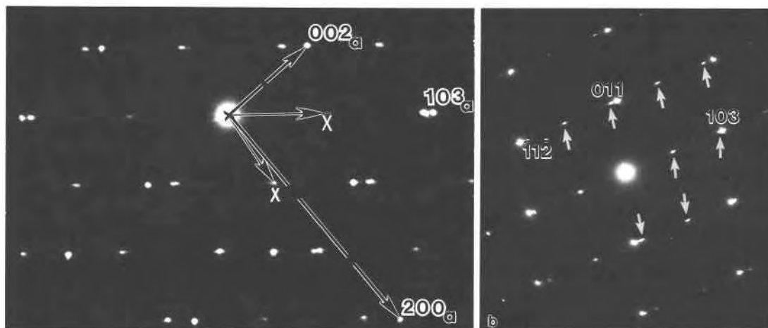
Fig. 3. SAED patterns (a) showing [010] of anatase and the reciprocal lattice from mineral X in lamellae coexisting with anatase; (b) in [3\bar{1}1] of anatase, showing the relative orientation of the two reciprocal lattices. Reflections from mineral X are arrowed.
