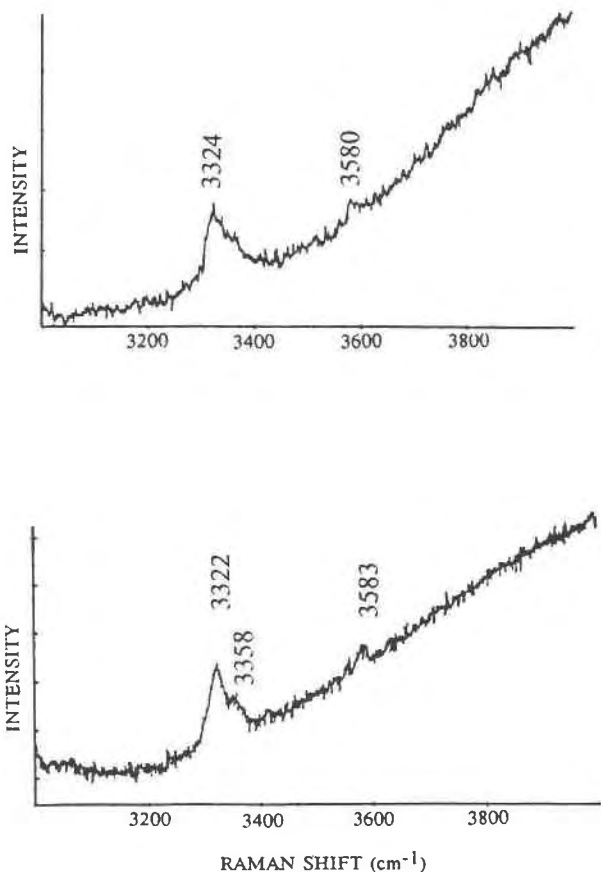
Fig. 2. Micro-Raman spectrum for a typical single grain of \beta -Mg 2 SiO 4 in the region 3000–4000 cm -1 , showing the fluorescence background and the features due to O-H stretching (top). The spectrum obtained previously (McMillan et al., 1987) for a polycrystalline aggregate of a similar sample is also shown for comparison (bottom).
