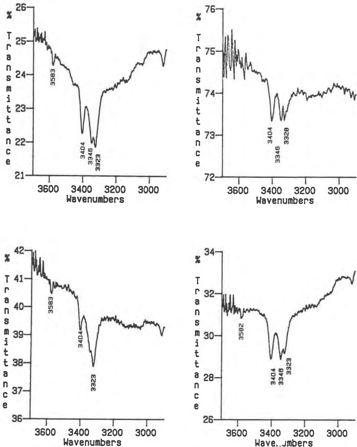
Fig. 4. Representative micro-IR spectra of \beta -Mg 2 SiO 4 grains in the O-H stretching region, obtained with a 15- \mu m aperture size, showing the variation in relative intensity of the peak at 3323 cm -1 , and the peaks at 3404 and 3346 cm -1 due to phase B.
