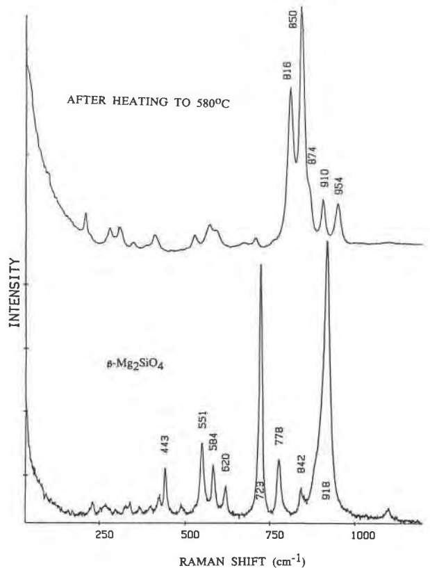
Fig. 9. Raman spectra of \beta -Mg 2 SiO 4 before (bottom) and after (top) heating to 580 °C for 5 min.
