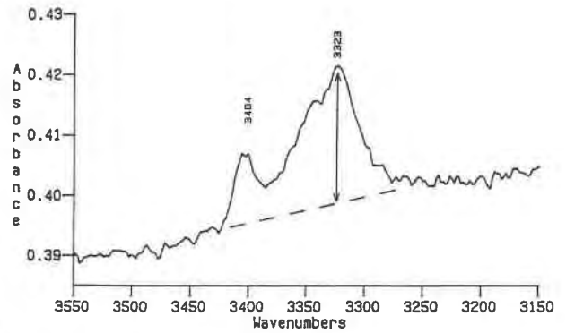
Fig. 8. Micro-IR absorbance spectrum of a large grain (approximately 10 \mu m across) of \beta -Mg 2 SiO 4 in the O-H stretching region, taken with a 15- \mu m aperture size. Other smaller grains (less than 1–2 \mu m) were also probably present in the field of view.
