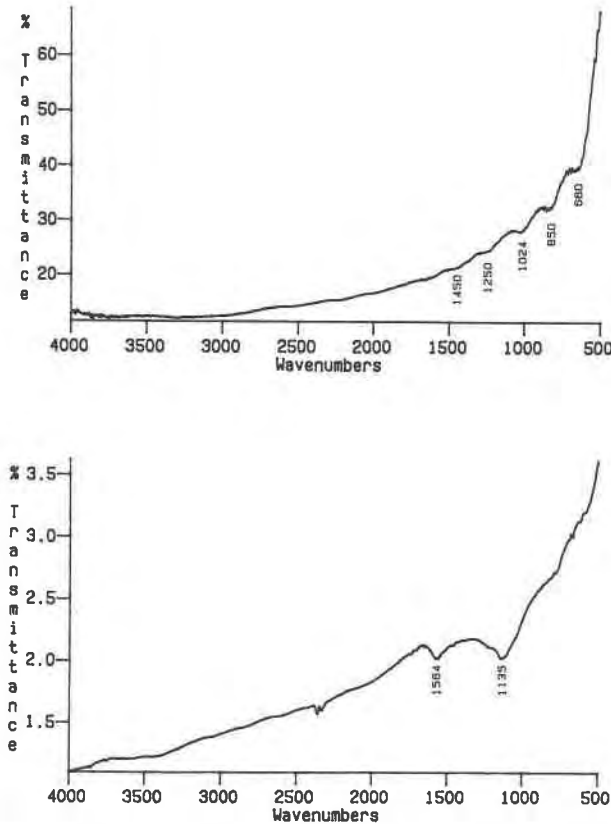
Fig. 7. Micro-IR spectra of crystalline graphite (top) and amorphous C black (bottom).
