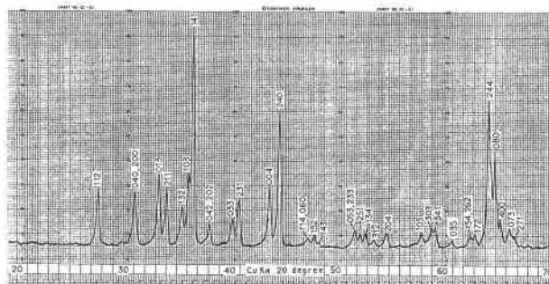
Fig. 1. Powder X-ray diffraction pattern for the sample of \beta -Mg 2 SiO 4 used in these studies.
