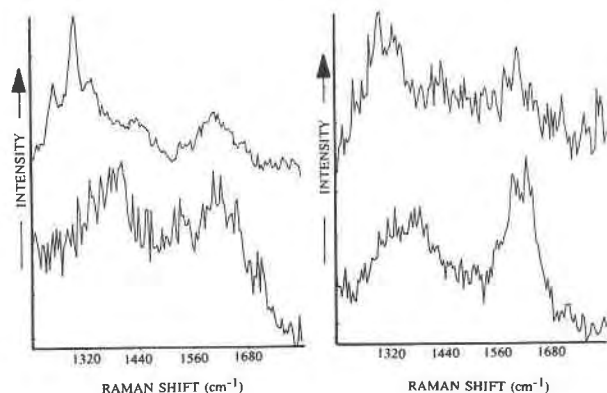
Fig. 6. Representative micro-Raman spectra for individual grains of \beta -Mg 2 SiO 4 in the region 1200–1800 \text{cm}^{-1} , showing the bands assigned to poorly crystallized graphite, presumably coating the samples.
