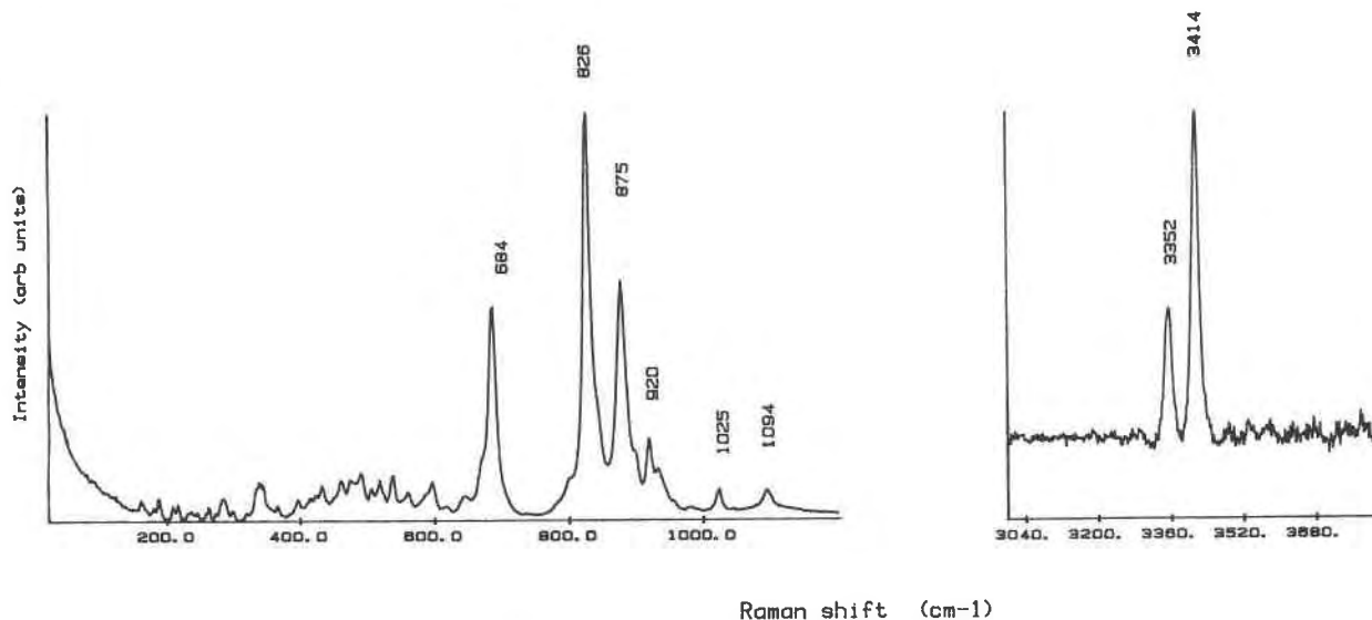
Fig. 5. Unpolarized micro-Raman spectra of phase B.
