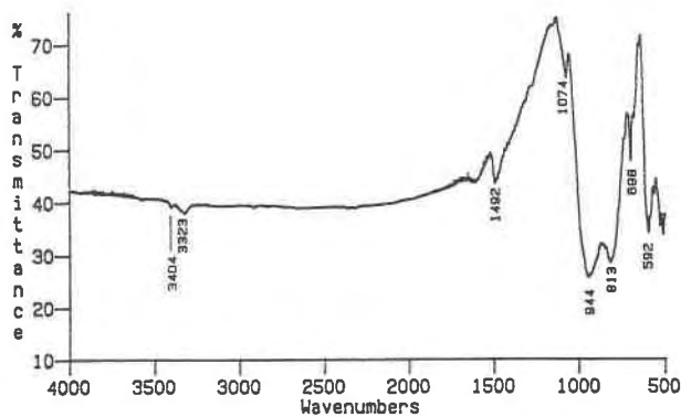
Fig. 3. Micro-IR spectrum of \beta -Mg 2 SiO 4 in the region 500–4000 cm -1 obtained with a 30- \mu m aperture. Several grains filled the field of view.
