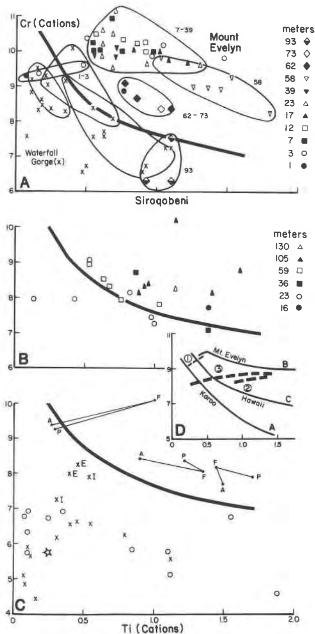
Fig. 9. Plot of Cr vs. Ti for chromite from different profiles from the Mount Ayliff Intrusion compared with analyses from elsewhere in the Karoo, from other intrusions, and from Hawaii. For reference, the trend for chromite from certain Hawaiian lavas (Wilkinson and Hensel, 1988) is shown as a heavy line. (A) Data for Waterfall Gorge (crosses) and Mount Evelyn, each sample from Mount Evelyn is designated separately and grouped stratigraphically. (B) Data for Siroqobeni profile. (C) Chromite from other Karoo intrusive rocks is shown by open circles (Eales and Snowden, 1979; Eales et al., 1980). Analyses from Rhum Intrusion are shown as crosses, those designated I are inclusions in olivine, E are external to olivine (Henderson and Suddaby, 1971; Henderson and Wood, 1981). Analysis of chromite in olivine from the Jimberlana Intrusion is denoted by a star (Roeder and Campbell, 1985). Samples joined and denoted F, A, and P are chromites enclosed in forsteritic olivine, plagioclase, and pyroxene, respectively, from individual samples from the Tabankulu lobe (Lightfoot and Naldrett, 1983). (D) Schematic and simplified trends for different suites of tholeiitic rocks. Karoo, Hawaii, and Mount Evelyn refer to typical trends displayed by chromites from these localities. Dashed trends 1, 2, and 3 refer to trends in the Mount Evelyn and Siroqobeni profiles (see text).
