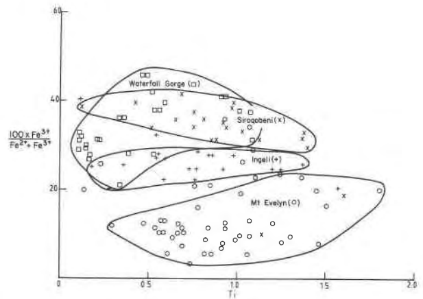
Fig. 7. Plot of 100 \times \text{Fe}^{3+}/\text{Fe}^{2+} + \text{Fe}^{3+} against Ti, based on 32 O anions for different profiles through Mount Ayliff Intrusion. Symbols as in Figure 3. All profiles show a similar range of Ti values, but 100 \times \text{Fe}^{3+}/\text{Fe}^{2+} + \text{Fe}^{3+} varies markedly.
