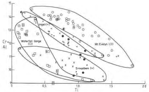
Fig. 4. Plot of cation Cr + Al vs. Ti for chromite compositions, based on 32 O anions. Symbols as in Figure 3.
