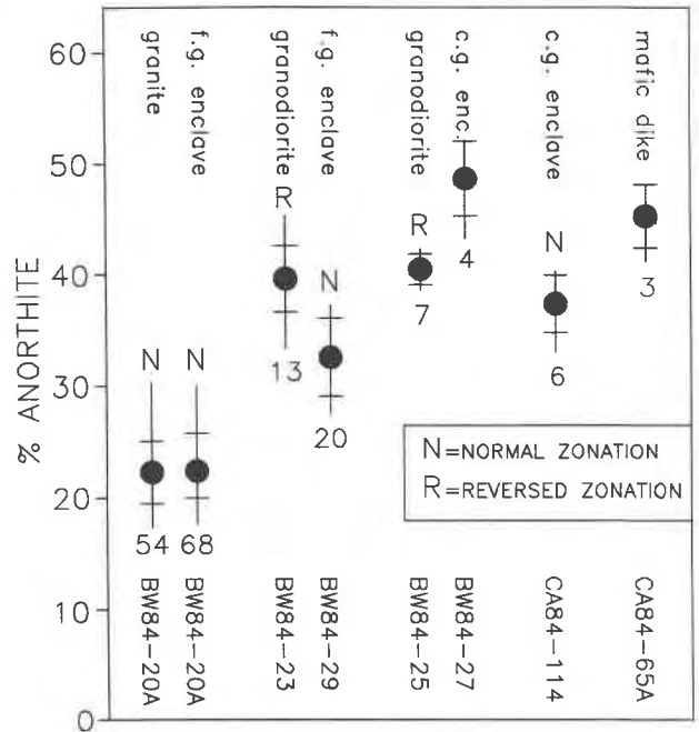
Fig. 11. Plagioclase compositions. Range is given by vertical line, 1 standard deviation by cross bars, and mean by dot. Number of analyses is given below the line. Host granitoid-mafic rock pairs are given together.
