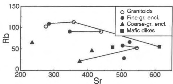
Fig. 7. Plot of Rb vs. Sr in ppm. Lines connect paired mafic rock-host granitoid samples.
