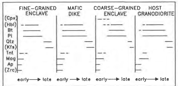
Fig. 6. Crystallization sequences for mafic rocks and granitoids. Minerals given in parentheses may be present or absent in a given sample.
