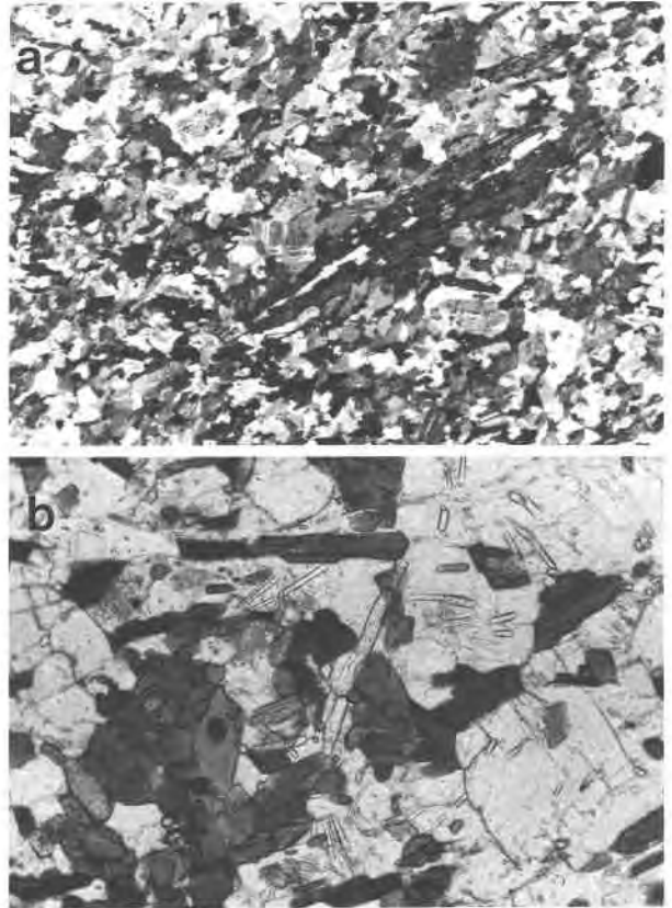
Fig. 5. Photomicrographs showing typical textures of fine-grained enclaves, particularly (a) hypidiomorphic-granular texture with acicular hornblende (photo 5 mm across), and (b) common acicular apatite, which is segmented in many cases (photo 1.8 mm across).
