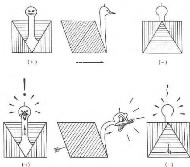
Fig. 1. Octahedra in pyriboles form strips along c , and have their symmetry planes parallel to (010) . With pyribole (100) horizontal, Thompson chooses pyribole stacking vectors parallel to c with their positive direction as that in which the ducks swim ( top row ). These stacking vectors correspond to the horizontal projections of standard mica stacking vectors, which, as Thompson points out, are “distinctly uncomfortable but not necessarily fatal” ( bottom row ). Adapted from Thompson (1981, Figs. 5 and 6).
