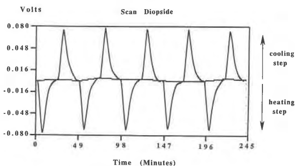
Fig. 2. Typical plot of voltage vs. time during ten alternating heating and cooling scanning steps. In this example, the diopside sample (equilibrated at 1624 K for 90 min) was initially heated at a rate of 1 K/min for 5 min followed by an isothermal interval of 20 min. The sample was then cooled at a rate of 1 K/min for 5 min followed by another isothermal period. Note that the baseline remained flat throughout all ten steps, indicating that the calorimetric detector was well balanced in terms of the heat capacities of the reference and sample chambers. The area under each peak was calculated, and the average of these ten values was taken as one datum.
