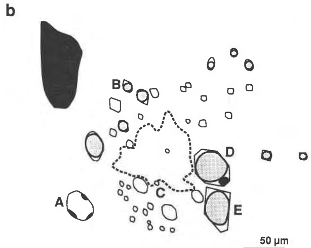
Fig. 5. (a) A cloud of fluid inclusions with peripheral larger inclusions with negative crystal shapes in the medium-grade sample (1021). See b for scale. (b) A sketch of the cluster of inclusions in a. White areas = \text{CO}_2 -rich inclusions; lightly shaded areas = vapor phase in aqueous inclusion; darkly shaded areas = solid phases; dashes = outline of the cloud of inclusions; A-E, see Table 1.
