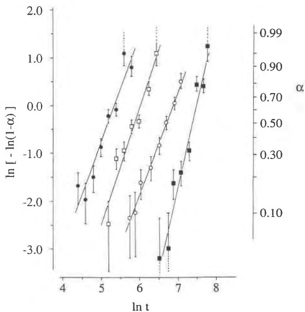
Fig. 4. Plot of \ln[-\ln(1 - \alpha)] against logarithm of time (in minutes). Measurements at 735 K are represented by filled circles, at 723 K by open squares, at 710 K by open circles, and at 698 K by filled squares.
