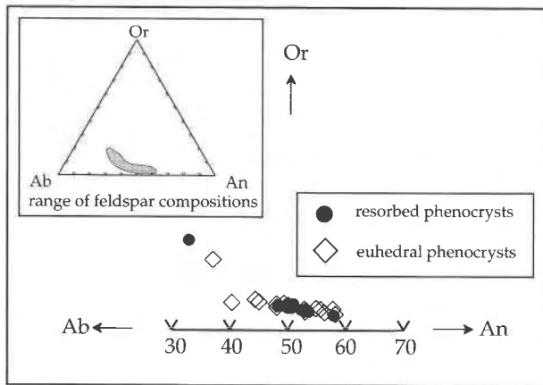
Fig. 7. Compositions of coexisting euohedral and resorbed phenocryst interiors from the lava in Figure 1.
