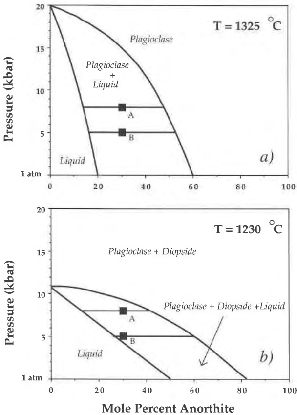
Fig. 2. (a) P - X section of the Ab-An system at 1325 °C (see Morse, 1980, Fig. 18.8). (b) P - X section of the pseudobinary plagioclase loop at about 1230 °C in the system Di-Ab-An constructed by moving the 1-atm loop up 100 °C to approximate its position at 10 kbar. This is a reasonable assumption, especially for the An-rich side of the diagram (see Morse, 1980, Figs. 18.6, 18.9). A given isothermal pressure drop produces a greater change in the composition and proportion of liquid in the system Di-Ab-An than in the system Ab-An.
