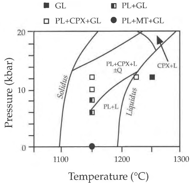
Fig. 3. P - T projection for andesite melts modified from Green (1972). Experimental phase assemblages from this study are also plotted for comparative purposes. Symbols the same as in Table 2.
