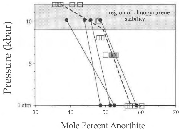
Fig. 4. Composition of plagioclase experiment products (open squares) as a function of pressure in terms of mole percent An, as determined by electron microprobe. Data from Meen (1987) (filled circles) are shown for comparative purposes where tie lines join plagioclase compositions from four starting materials under nearly isothermal ( \sim 1150 °C) conditions. Dashed line illustrates that the change in plagioclase composition may vary more strongly with pressure when clinopyroxene is stable.
