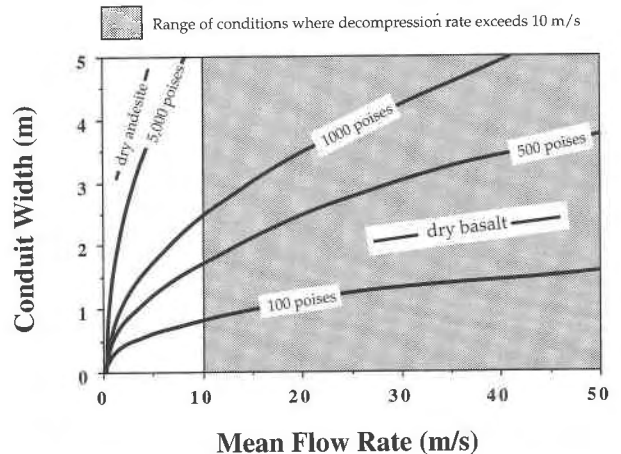
Fig. 6. Curves of mean flow rate or ascent rate of magma through a dikelike conduit as a function of conduit width and magma viscosity for a density contrast of 0.2 g/cm 3 between the wall rock and magma (Kushiro, 1980, p. 117). Approximate values for dry andesite and basalt are shown for comparison. Note that ascent rates of >10 m/s (shaded region) are easily achieved for a reasonable range of geologic conditions in this model.
