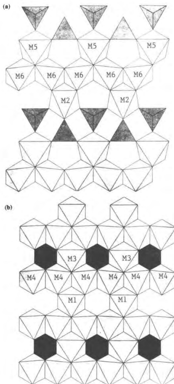
Fig. 1. Two types of (010) layers in the anhydrous phase B structure reveal a possible rationalization for extensive Mg-Fe ordering. Olivine-type layers (a) contain M2, M5, and M6 octahedra, all enriched in Mg. The (b) layers, on the other hand, contain Si octahedra surrounded by Mg-Fe octahedra. The Fe-rich site, denoted M3, is the only octahedron to share edges with two octahedral Si sites (in black). This concentration of Fe creates two chemically distinct kinds of edge-sharing octahedral strips parallel to a . Predominantly Mg sites form strips with equally sized M6 or M4 octahedra. Enclosed by these chains are strips in which smaller Si and larger (Mg,Fe) octahedra alternate. The concentration of larger Fe cations in the latter strips compensates for the smaller Si octahedra.
