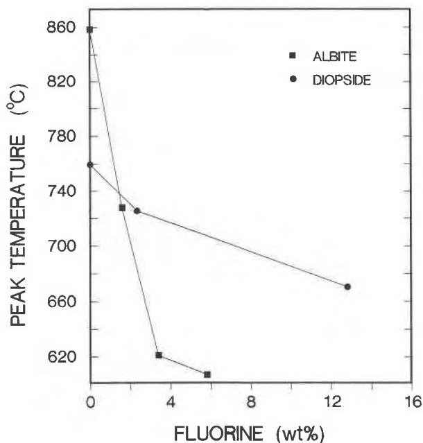
Fig. 3. The effect of F on the glass transition of diopside and albite melts as indicated by the peak temperature of glasses cooled and subsequently reheated at 5 K/min.
