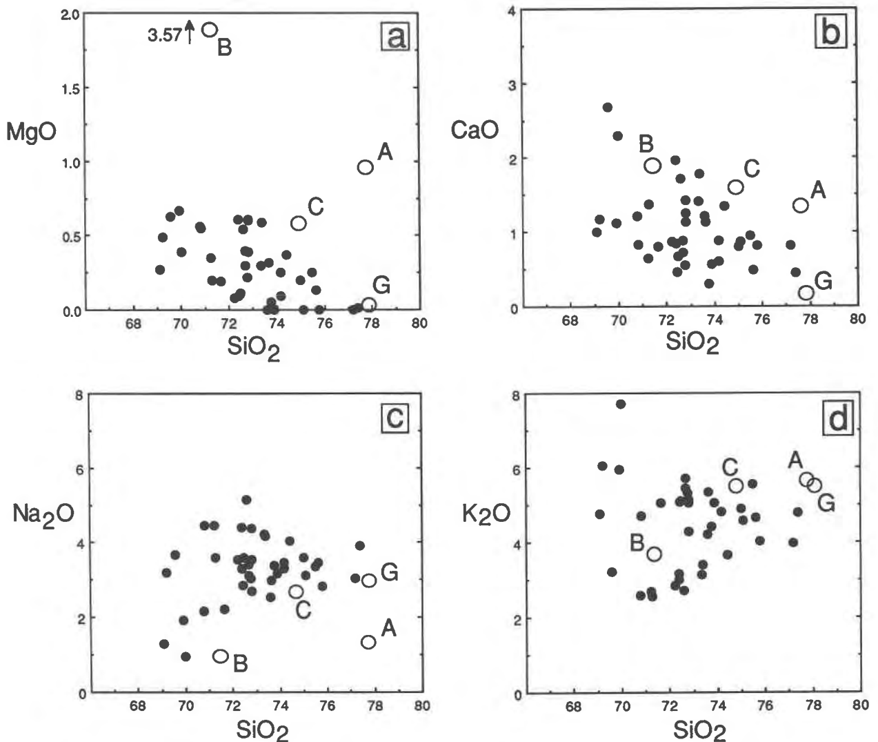
Fig. 17. Diagrams of variations in element concentrations for bulk analyses from silicic pyroclastic tuffs. Data taken from literature sources are solid circles; Lovelock layers A, B, and C, as well as the fresh Lovelock glass (G) in layer C, are represented by large open circles.
