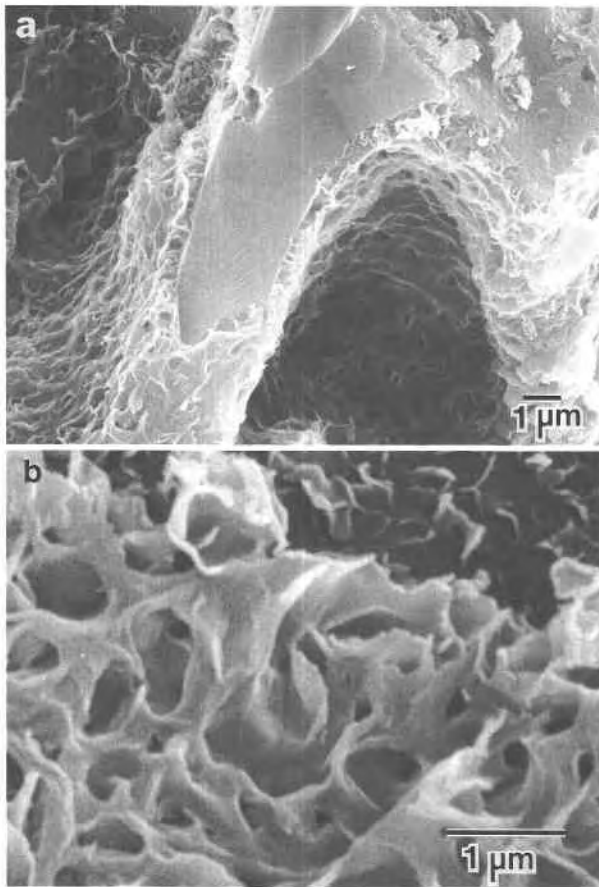
Fig. 4. SEM micrograph showing (a) a fracture section of glass in sample SR75 and (b) the morphology of smectite on the glass surface.
