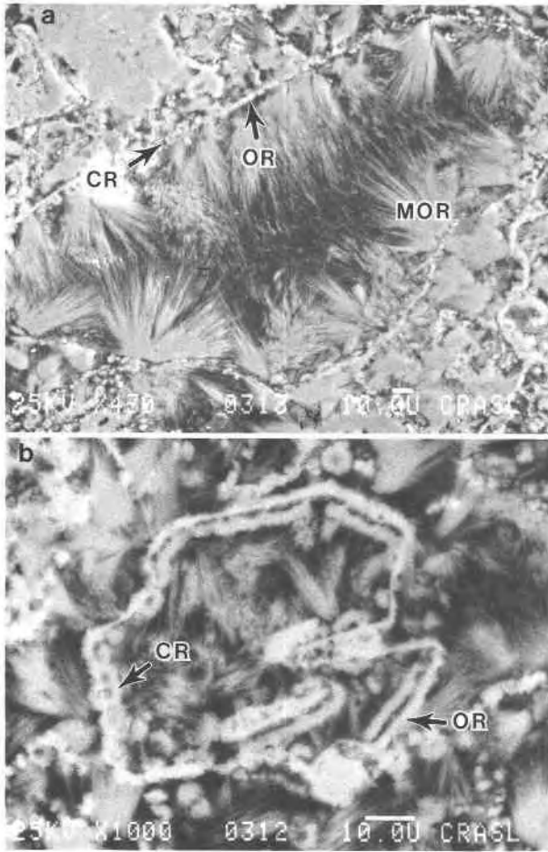
Fig. 12. Cross sections of mordenite tuff SR3 showing (a) individual void space, outlined by orthoclase crystallite network and partially filled with prismatic mordenite, (b) double-walled texture of orthoclase and minor cristobalite.
