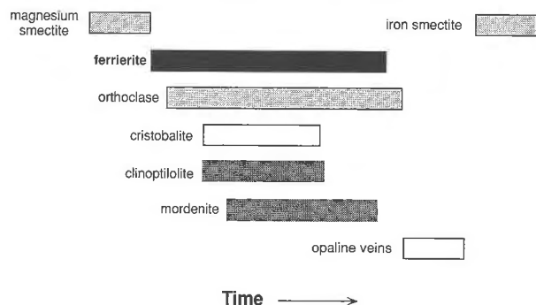
Fig. 13. Paragenetic sequence of authigenic minerals recognized in the Lovelock deposit.
