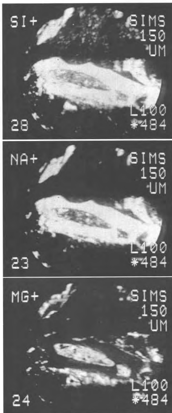
Fig. 5. SIMS images of a polished section of vitric tuff sample C3-30.5. The Si image identifies the shape of the glass shard. The Na image, which imitates Si here, confirms that alkalis are uniformly present in the glass and therefore leaching has not occurred. The Mg is a constituent of the smectite coating the glass.
