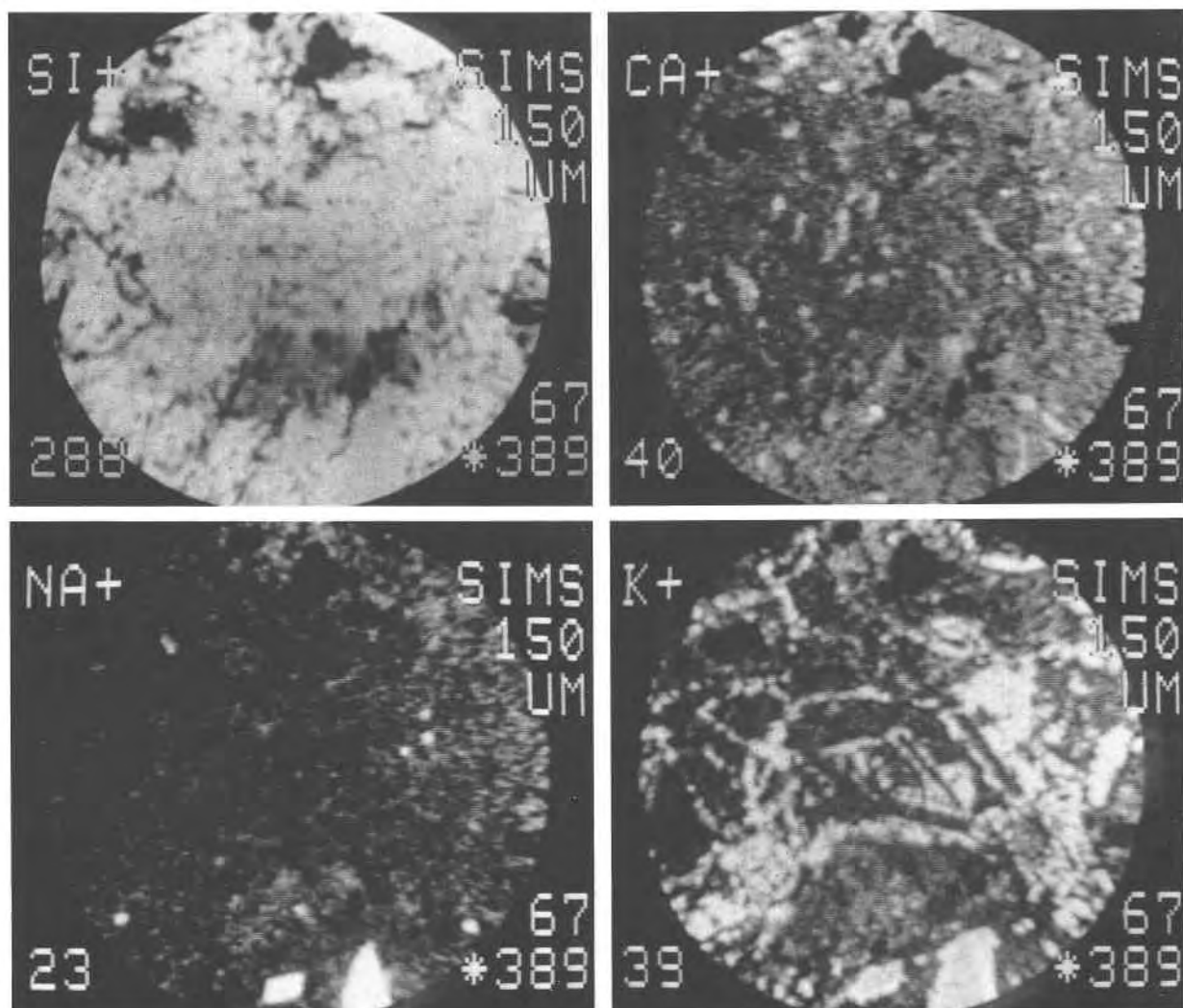
Fig. 11. SIMS images of a cross section of sample SR67. Most of the areas of high K concentration represent orthoclase. The two grains in the bottom of the field are sanidine pyroclastic grains.
