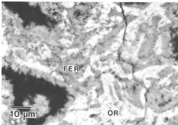
Fig. 9. Backscattered electron image of cross section of densely intergrown ferrierite and orthoclase (ferrierite tuff SR67), the latter showing the relict shard position.
