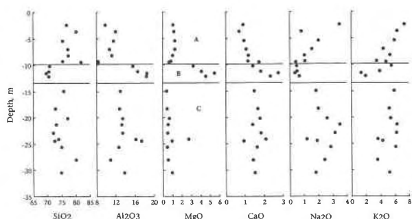
Fig. 14. Variation of element concentrations with depth in hole no. 3 tuffs. Layer A is predominantly ferrierite and orthoclase. Layer B is predominantly ferrierite and smectite. Layer C is glass and clay.
