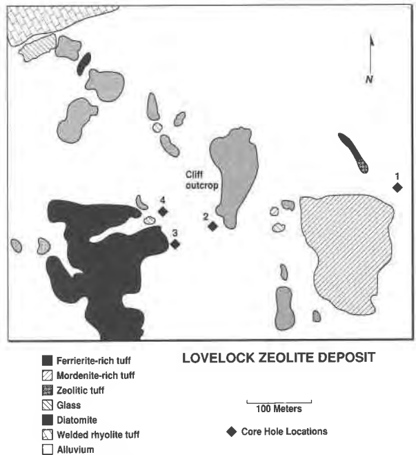
Fig. 2. Geologic map of the Lovelock deposit.
