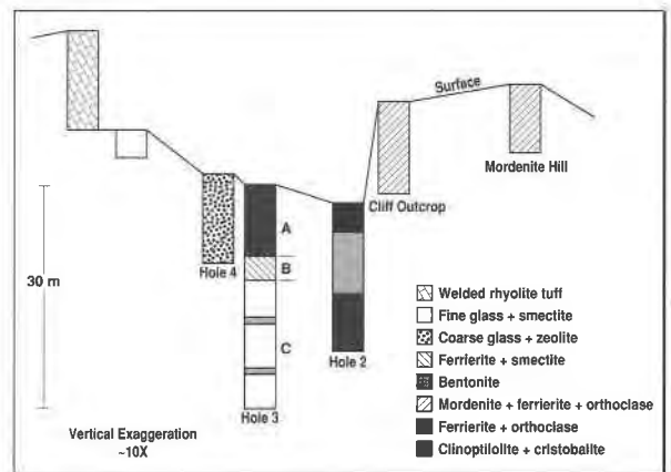
Fig. 3. Stratigraphy of the Lovelock zeolite deposit. Layers A, B, and C are defined on the basis of composition (as in Fig. 14) and assemblage.
