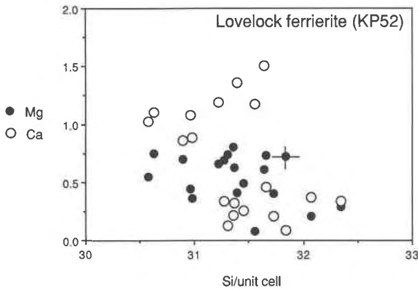
Fig. 15. Divalent cation concentrations vs. Si for individual ferrierite crystals from a small chip of ferrierite tuff (KP52). Data were obtained from TEM/EDX analyses, based on unit-cell contents of 72 O atoms.
