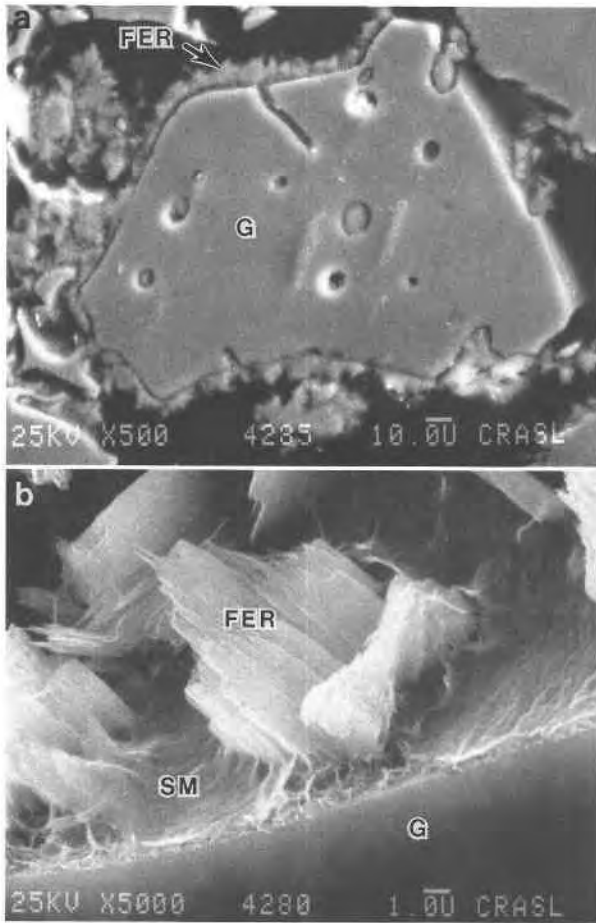
Fig. 8. (a) Cross section of a single glass shard (G) with ferrierite at its periphery. (b) Higher magnification image of ferrierite (FER) and smectite (SM) adjacent to the glass. Microanalysis and morphology confirmed the identity of ferrierite.
