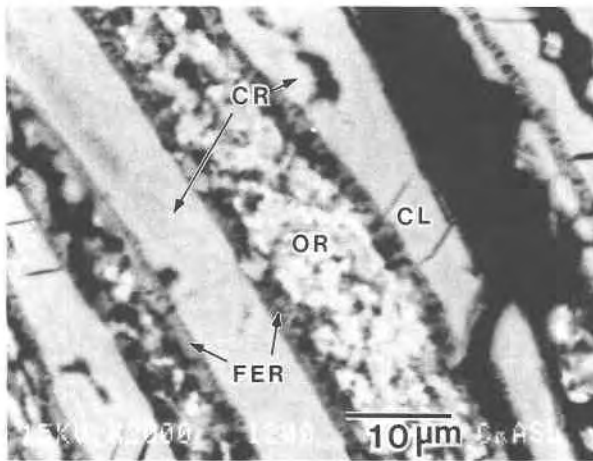
Fig. 6. Backscattered electron image of a cross section of sample C2-3.7 showing replacement of glass by clinoptilolite (CL) and cristobalite (CR). Ferrierite (FER) and orthoclase (OR) formed between the limbs of the shard. Some of the ferrierite has grown normal to the former glass surface. Note also that cristobalite spheroids occur as discrete crystallites within the limbs.
