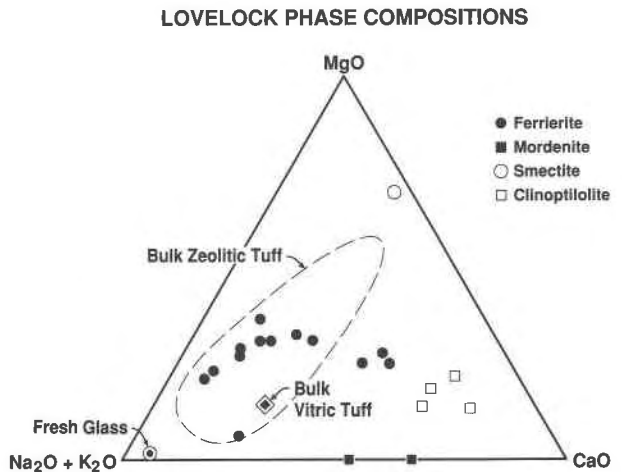
Fig. 16. Normalized MgO-(Na 2 O + K 2 O)-CaO contents (wt%) for Lovelock zeolites and tuffs. The dashed field represents about 40 bulk analyses of tuffs from Lovelock.
