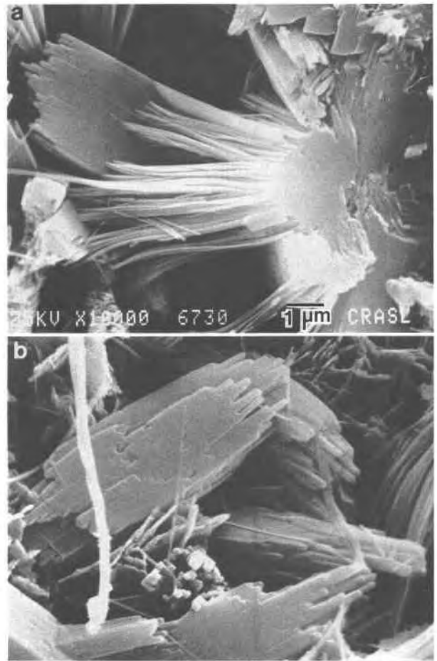
Fig. 10. Fracture section of sample SR67 showing ferrierite habits. (a) Radiating bundle of fibers. (b) Boxy acicular crystals.
