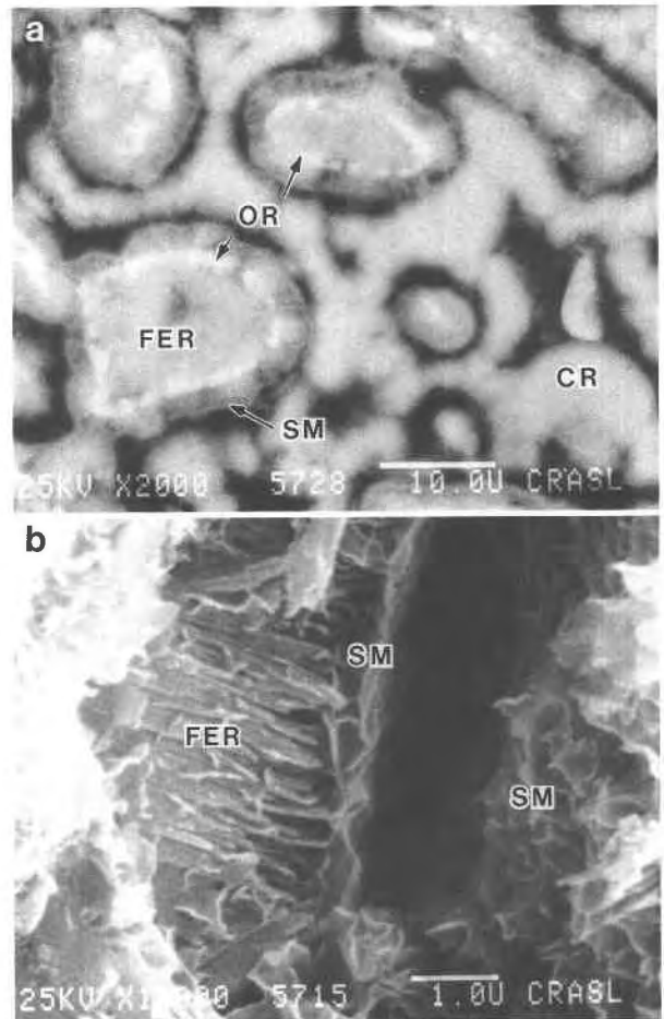
Fig. 7. (a) Back-scattered electron image of sample C2-17.4 showing orthoclase (OR), ferrierite (FER), and smectite (SM) filling the pores of a relict shard. The shard walls are the connected curvilinear features separating rounded pores. Some of this wall material is now cristobalite (CR). (b) Fracture section of sample C2-17.4 showing empty pore space (black) rimmed by smectite and ferrierite.
