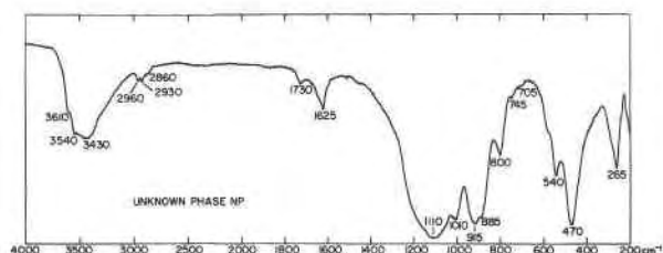
Fig. 9. Infrared spectrum of new alkali uranyl silicate (NP) phase.
