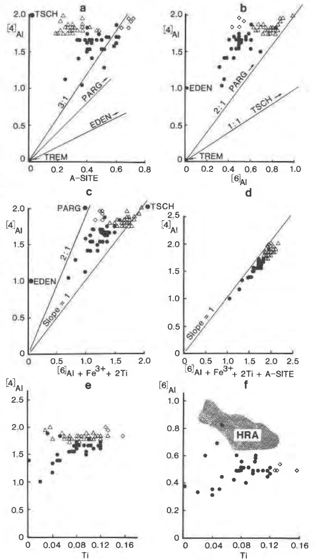
Fig. 4. Variation of amphibole compositions (solid circles = Davis Mill samples, triangles = Hudson Mill Rapids, and diamonds = Lindsey Creek. End-member abbreviations: PARG = pargasite; EDEN = edenite; TSCH = tschermakite; TREM = tremolite). (a) Plot of [4]Al vs. A site [^{14}(Na + K)] . (b) Plot of [4]Al vs. [6]Al illustrating deviation of amphibole compositions from a line of slope 1 indicating a tschermakite substitution vector. (c) Plot of [4]Al vs. [6]Al + Fe^{3+} + 2Ti showing M2-site substitution. (d) Plot of [4]Al vs. [6]Al + Fe^{3+} + 2Ti + A site illustrating the effect of A-site substitution. (e) Plot of [4]Al vs. Ti showing uniform [4]Al for Hudson Mill Rapids and Lindsey Creek relative to Davis Mill amphibolites. (f) Plot of [6]Al vs. Ti showing a general inverse relationship for Hudson Mill Rapids (ruled field, HRA) but not for Davis Mill amphibolites.
