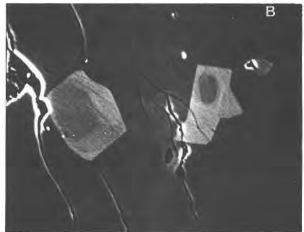
Fig. 10. (A) Backscattered electron image of zoisite and clinozoisite, together with albite (black, unlabeled), (B) 20- \mu\text{m} inclusions of clinozoisite in zoisite (close-up of the left central part of the zoisite crystal in A). Matrix and inclusion clinozoisite show the same type of zoning (sample RM71).
