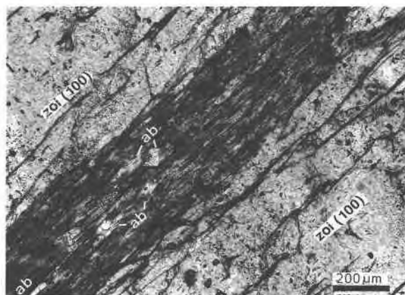
Fig. 7. Photomicrograph of zoisite with 10–12 mol% \text{Al}_2\text{Fe} with alteration zones parallel to (100) (dark because of anomalous interference colors) with 15 mol% \text{Al}_2\text{Fe} , intergrown with albite (ab; sample 85-1, crossed polars).
