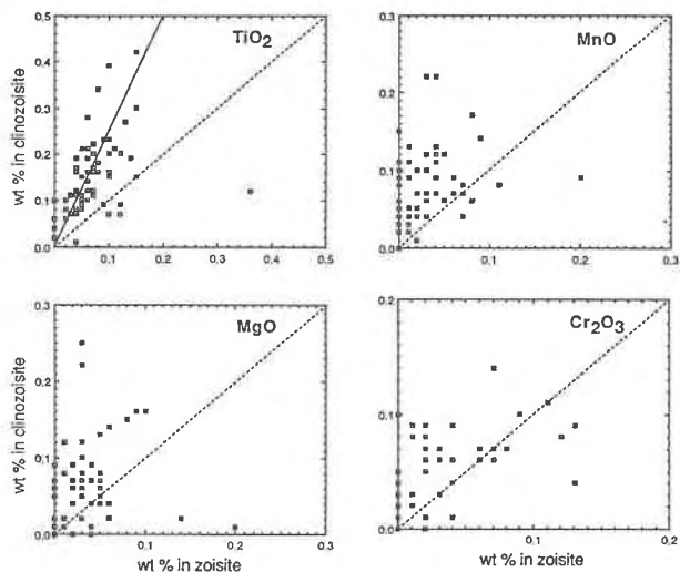
Fig. 4. Distribution of the minor components \text{TiO}_2 , \text{MnO} , \text{MgO} , and \text{Cr}_2\text{O}_3 between clinozoisite and zoisite (same data set as Fig. 3; overlapping analyses not shown). The 1:1 slope line is given as a reference line; for \text{TiO}_2 a reference line with a slope of 2.5:1 is also shown.
