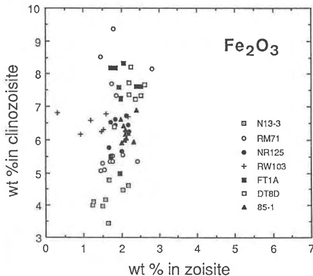
Fig. 3. Distribution of \text{Fe}_2\text{O}_3 between clinozoisite and zoisite (only analyses of grains in contact with one another are plotted); clinozoisite is strongly enriched in \text{Fe}_2\text{O}_3 .
