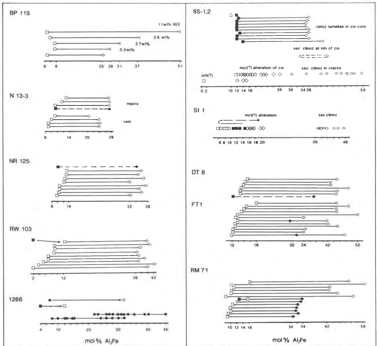
Fig. 5. Analytical results for the investigated samples of clinzoisite-zoisite pairs; squares = orthorhombic; diamonds = monoclinic; rotated squares = structural state uncertain; triangles = rare earth-bearing clinzoisite. Lines connect coexisting minerals; analyses were made a few micrometers away from the grain boundary. Sample BP 119: REE-bearing and REE-free inclusions of clinzoisite in zoisite; the width of the two-phase area widens with increasing REE content. N 13-3: Matrix and vein assemblage in a low-grade amphibolite; filled symbols indicate core compositions. Sample NR 125: Tourmaline-epidote segregation from contact metamorphic environment; filled symbols indicate core compositions. Sample RW 103: Calc-silicate nodule from a polymetamorphic granulite to amphibolite facies terrane. Solid symbol indicates Fe-poor granulite facies zoisite with overgrowth of Fe-richer zoisite during amphibolite facies metamorphism. Sample 1266: Low-grade calc-silicate rock. Closed and open squares represent core and rim analyses, respectively, of grains determined optically to be orthorhombic; closed and open diamonds are core and rim analyses from clinzoisite, with a continuous range of intermediate compositions (no analysis points shown). Closed diamonds (lower two rows) represent monoclinic intergrowths (two crystals determined with TEM) that contain 8–32 mol% Al_2Fe in one case and 22–46 mol%
