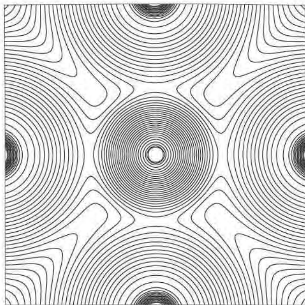
Fig. 6. A total electron density map calculated through a plane defined by Na and four Cl atoms in a \text{NaCl}_6 octahedron. The map was calculated using the sum of the electron densities from spherically averaged atoms calculated from the Roothaan-Hartree-Fock wave functions (Clementi and Roetti, 1974). The k th contour, counting from the corners of the map, corresponds to the value (3.0 \times 10^{-4})(1.3^{k-1})e/b^3 . The contours at the atom centers have been omitted.
