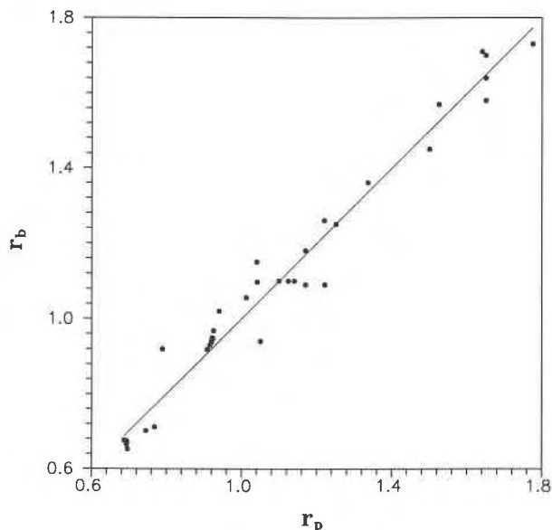
Fig. 8. Bonded radii, r_b , obtained from experimental electron density distributions measured for NaCl, RbCl, LiF, KCl, KBr, coesite, stishovite, MgO, NiO, CuCl, CuBr, BeO, and CaF 2 vs. promolecule radii, r_p , calculated for the nonequivalent coordination polyhedra in each of these crystals with the bond lengths and angles fixed at observed values.
