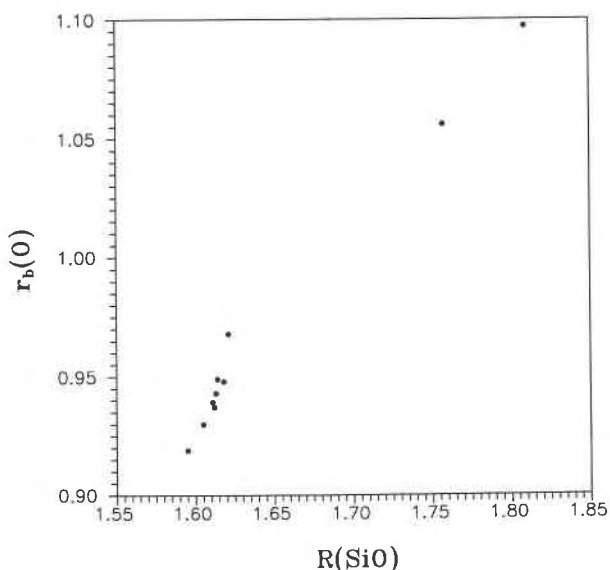
Fig. 2. The bonded radius of the oxide ion, r_b(\text{O}) , measured from static electron density maps, provided by pseudoatom refinements of observed diffraction data for coesite and stishovite vs. the observed SiO bond length, R(\text{SiO}) , in angstroms. The pseudoatom refinements were completed by Geisinger et al. (1987) and Spackman et al. (1987), and the bonded radii were measured by Buterakos (1990).
