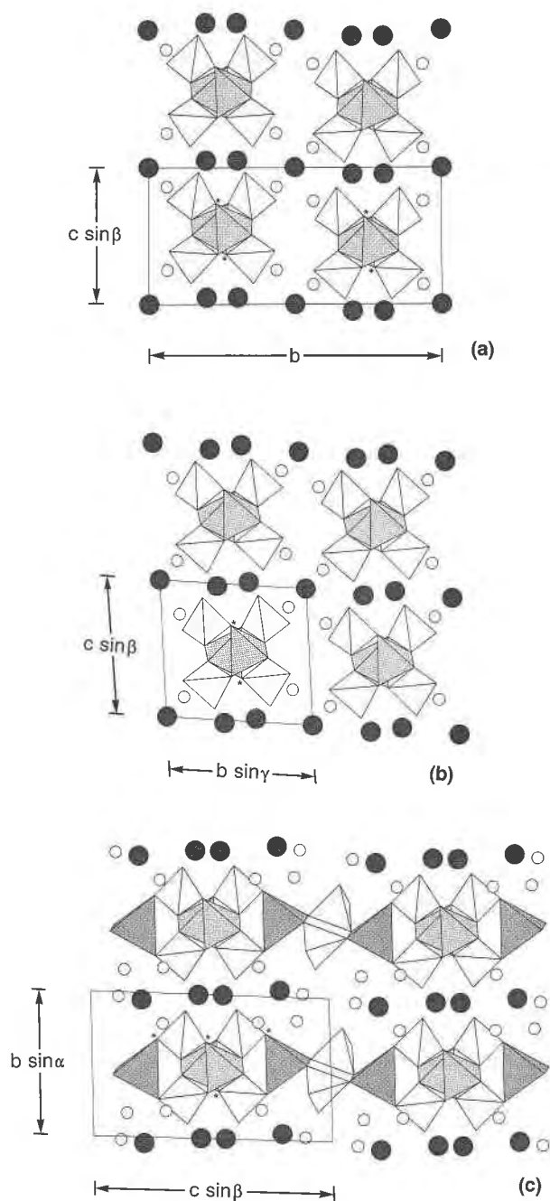
Fig. 2. The structures of (a) fransoletite, (b) parafransoletite, and (c) ehrleite, all projected down [100]. The BeO 4 tetrahedra overlap one another. Asterisks indicate apparent tetrahedral joins; the tetrahedra are actually attached to corresponding tetrahedra above or below.
