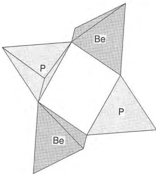
Fig. 3. The four-membered ring of alternating BeO 4 and PO 4 tetrahedra found in the structures of numerous beryllophosphates.
