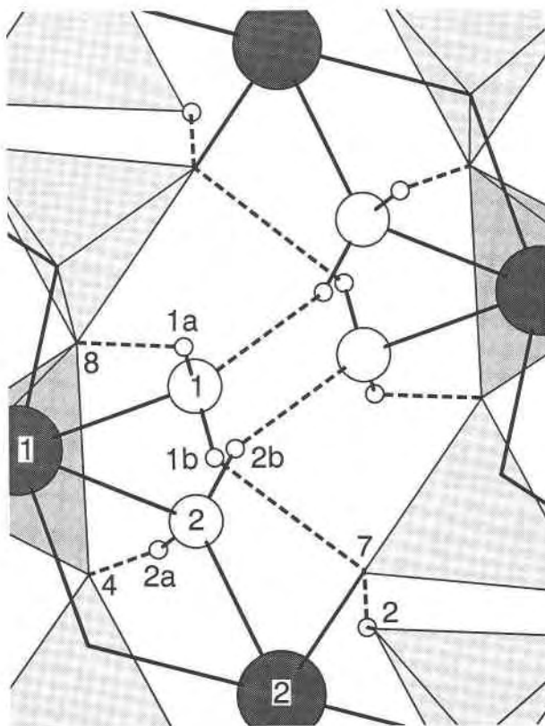
Fig. 4. Bonding in a portion of the parafransoletite structure projected along [001]. Darkly shaded circles are Ca atoms, large unshaded circles are H 2 O O atoms, and small unshaded circles are H atoms. The Ca-O and O-H bonds are shown as solid lines; H bonds are shown as dashed lines.
