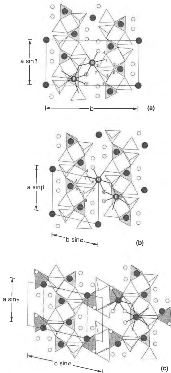
Fig. 1. The structures of (a) fransoletite and (b) parafransoletite, both projected along [001], and (c) ehrleite projected along [010]. Darkly shaded circles are Ca atoms, unshaded circles are H 2 O O atoms. In a and b, number labels are shown for Ca atoms (1 and 2), H 2 O O atoms (1 and 2), and tetrahedral O atoms (1-8). Bonds surrounding one Ca1 and one Ca2 atom in each structure are shown. The BeO 4 tetrahedra are located directly beneath Ca1 atoms. The Ca2 atoms in ehrleite partially overlap the ZnO 4 tetrahedra. A solid line outlines the unit cell in each structure. The dotted outline on the ehrleite drawing approximates the parafransoletite cell.
