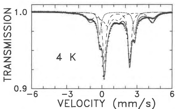
Fig. 2. Mössbauer spectrum of polycrystalline \text{Mg}_{0.957}\text{Fe}_{0.1}\text{SiO}_3 orthopyroxene at 4 K showing the onset of magnetic ordering. The solid line through the experimental points is a least-squares fit to the data, with the model including the full spin Hamiltonian described in the text. Three spectral sites are assumed present, one magnetic and two nonmagnetic. The computed sub-spectra correspond to nonmagnetic M1, nonmagnetic M2, and magnetic M2 sites, respectively (cf. Fig. 1). The magnetic interaction is due to spin-spin relaxation, but the fitting was performed assuming a static field with artificially broad lines.
