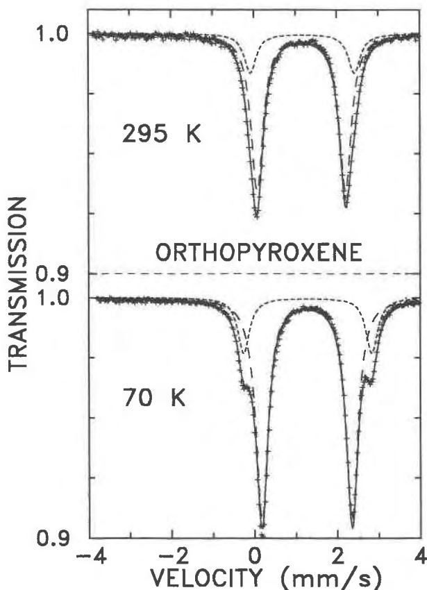
Fig. 1. Mössbauer spectra of polycrystalline \text{Mg}_{0.957}\text{Fe}_{0.1}\text{SiO}_3 orthopyroxene at 295 and 70 K are shown relative to Fe metal and corrected to a room-temperature source. Fits to the M1 and M2 doublets and the total spectrum are indicated by short- and long-dashed curves and by a solid curve, respectively.
