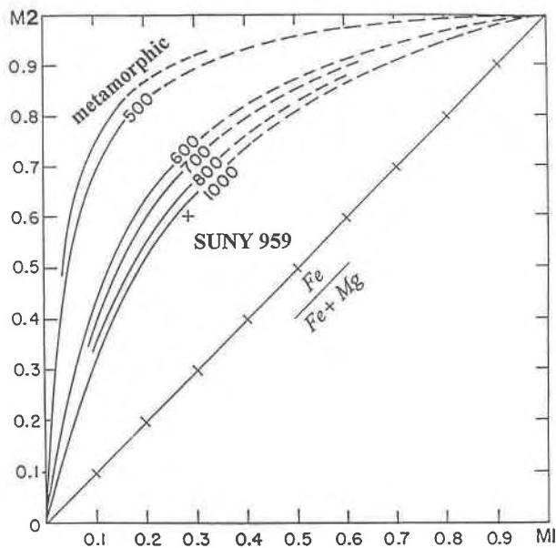
Fig. 1. The 11.3 GPa orthopyroxene single crystal described in this study plots slightly above the 1000 °C ordering isotherm of Virgo and Hafner (1969).
