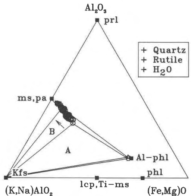
Fig. 13. Condensed AKM plot of analyses of primary (circles) and recrystallized (squares) muscovite, high-Ti (Ti > 0.3 atoms pfu; circle) matrix, and intergrown (star) biotite (Table 1), projected through \text{SiO}_2 , \text{TiO}_2 , and \text{H}_2\text{O} , and showing the schematic phase relations (KMASH system) relevant to primary muscovite decomposition [abbreviations as in Fig. 12, except Al-phl: aluminum phlogopite, \text{K}_2^{16}\text{Al}_3\text{Mg}_5\text{Al}_3\text{Si}_5\text{O}_{20}(\text{OH})_4 ]. The three-phase field A, defined by potassium feldspar, muscovite bearing the maximum Si content (6.66 atoms pfu), and high titanium matrix biotite represents the early equilibration assemblage. As decomposition of primary muscovite proceeds, the three-phase field expands (arrow), as represented by the three-phase field B defined by potassium feldspar, low-Si primary muscovite and intergrown biotite. The compositional deviations of muscovite undergoing decomposition from the ms-lcp join toward pyrophyllite and phlogopite end-members would produce less potassium feldspar upon decomposition relative to the amounts predicted by Reaction 1 (note also that the deviations of muscovite due to the Tk and Ti-Spl exchanges are collinear due to the projection through \text{TiO}_2 ). When projected into this diagram, the compositions of the heterogeneous matrix biotite overlap the aluminous biotite end-member.
